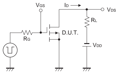
Fig.15 Switching Time Measurement Circuit
