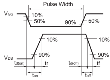
Fig.16 Switching Waveforms
