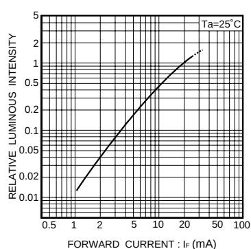
Fig.22 Luminous intensity vs. forward current
