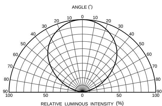
Fig.1 Directional pattern
