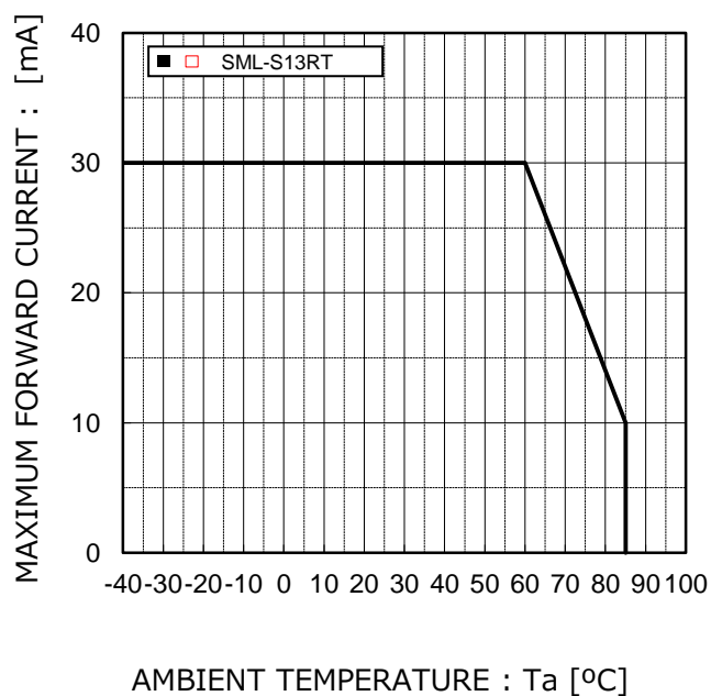
Fig.4 Derating
