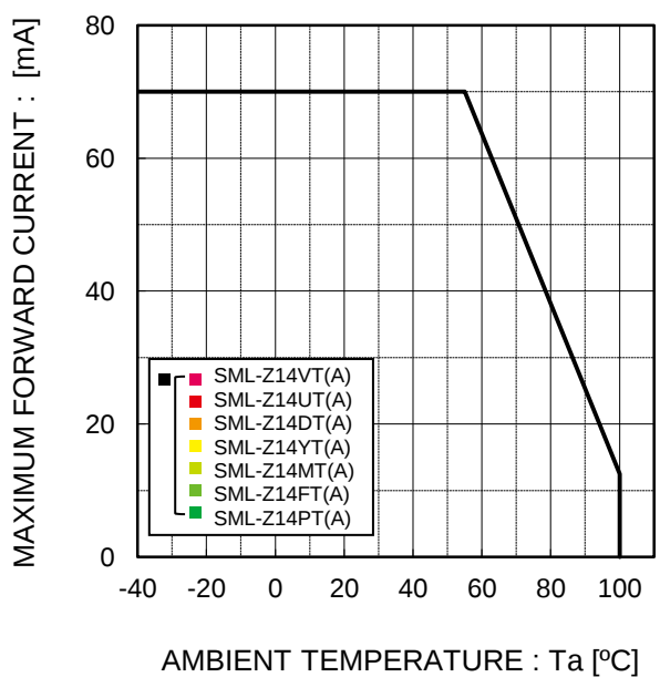
Fig.4 Derating
