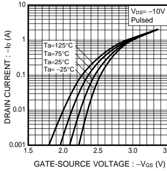
Fig.1 Typical Transfer Characteristics
