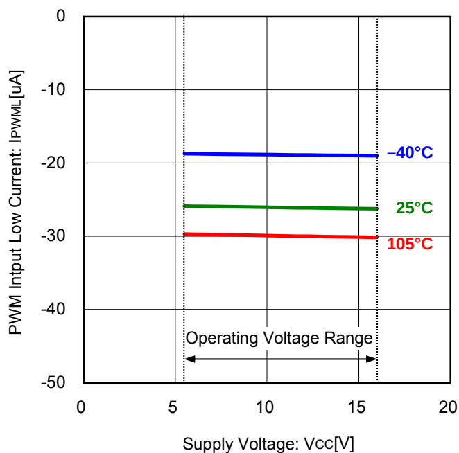
Figure 16. PWM Input Low Current vs Supply Voltage
