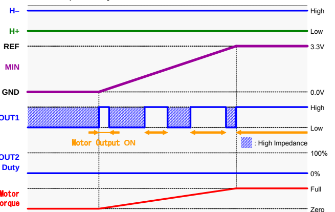
Figure 34. DC Input Operation Timing Chart
