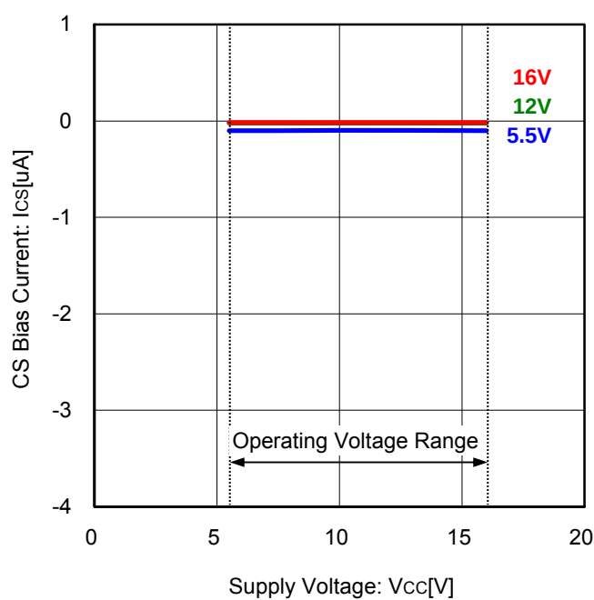
Figure 22. CS Input Bias Current vs Supply Voltage
