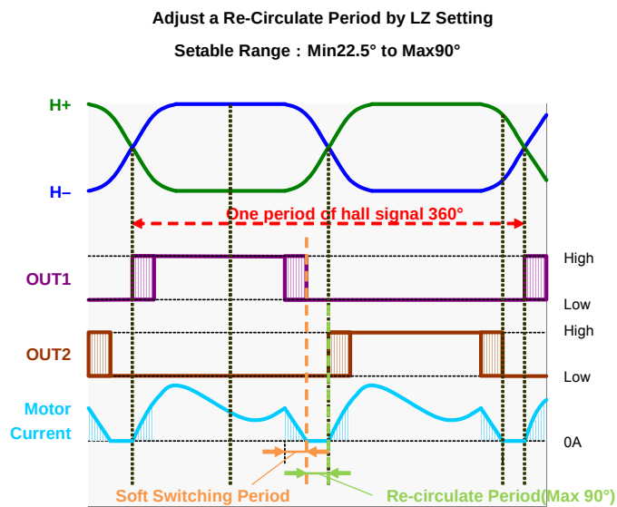
Figure 39. Recirculate Period Setting
