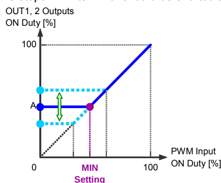
Figure 27. Setting of Minimum Output Duty
