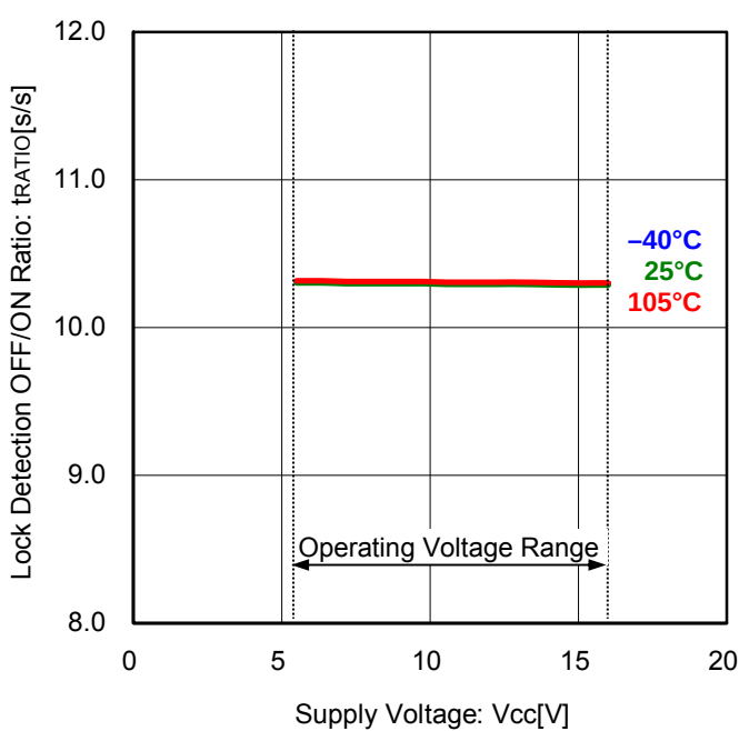
Figure 10. Lock Detection OFF/ON Ratio vs Supply Voltage
