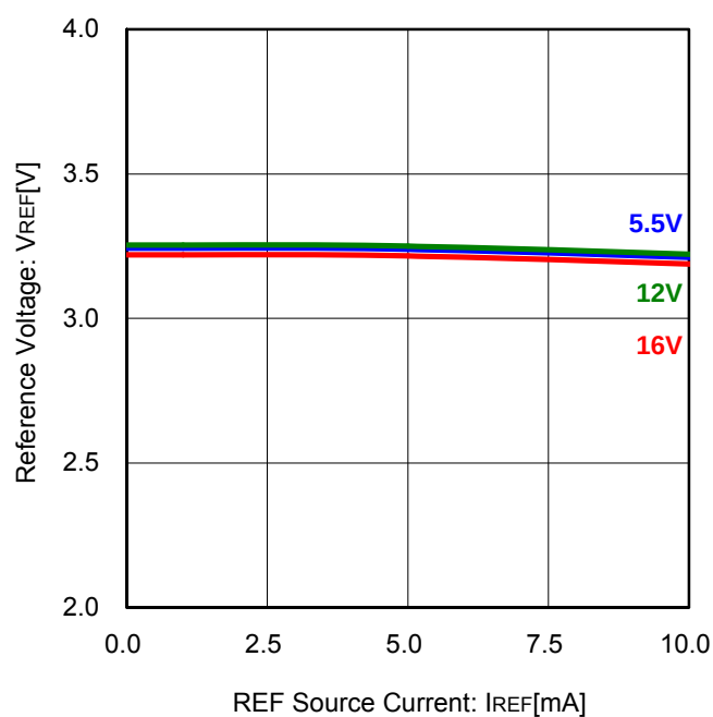
Figure 18. Reference vs REF Source Current (VCC=12V)
