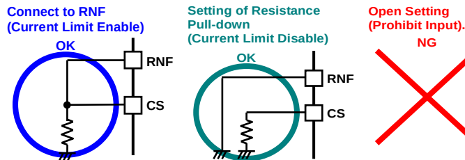
Figure 45. CS Terminal Setting
