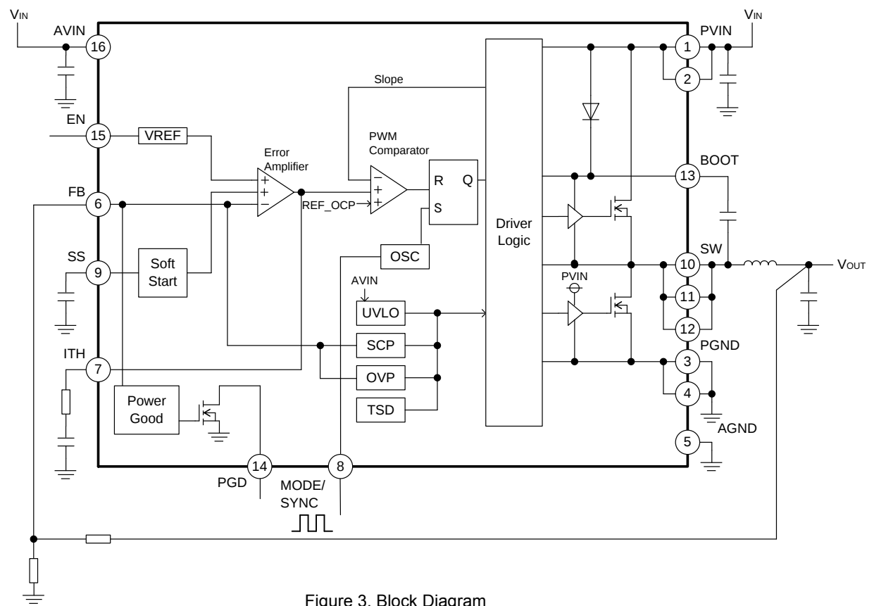
Figure 3. Block Diagram
