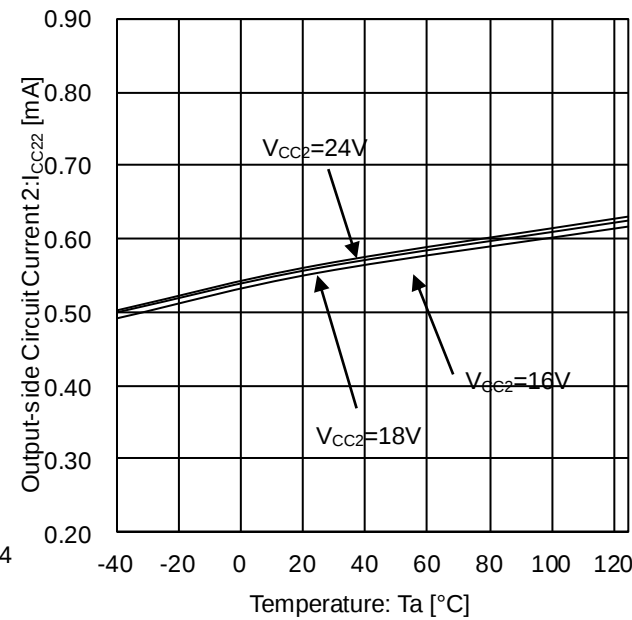
Figure 14. Output-side Circuit Current 2 vs Temperature (At OUT=H )
