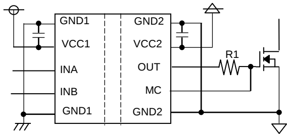
Figure 31. Driving SiC
