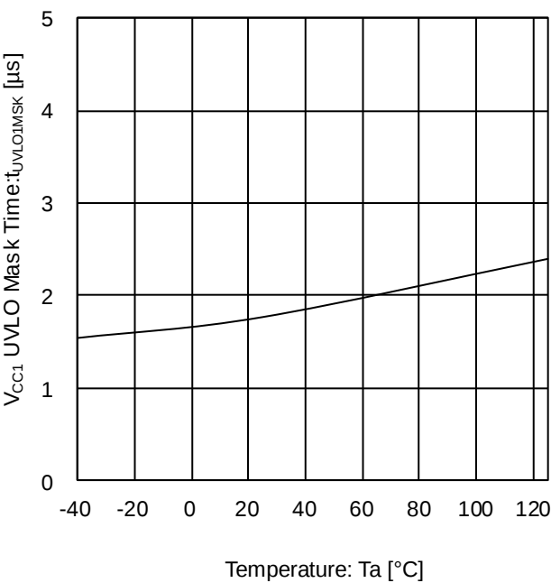
Figure 28. V CC1 UVLO Mask Time vs Temperature
