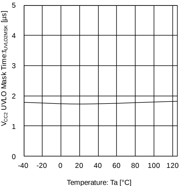
Figure 30. V CC2 UVLO Mask Time vs Temperature
