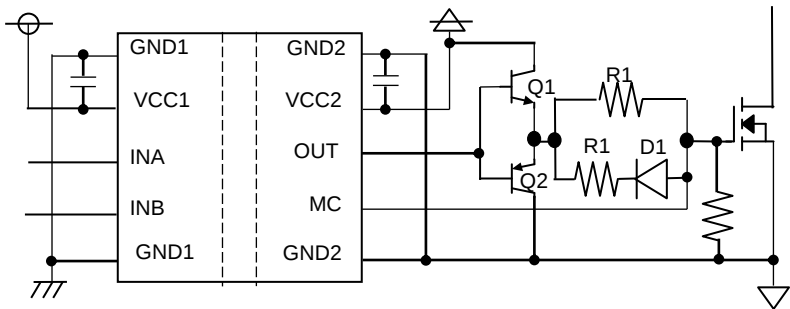
Figure 32. Driving SiC with Buffer Circuit
