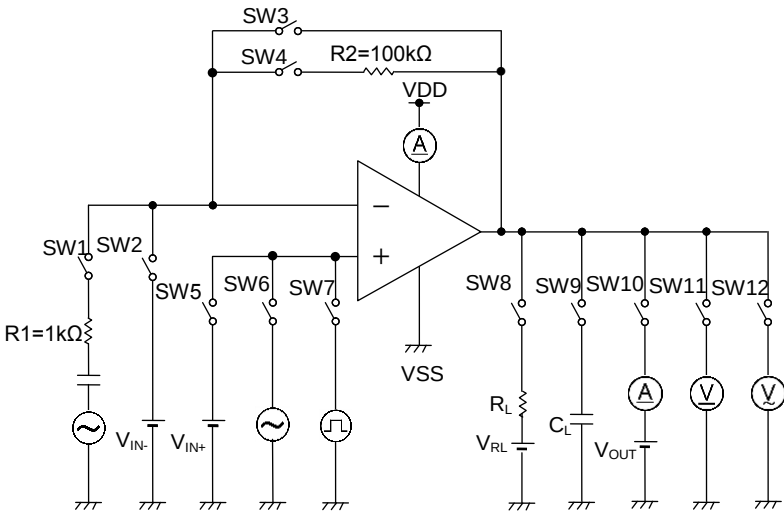
Figure 31. Test Circuit 2
