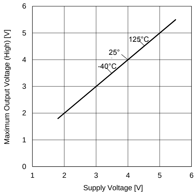
Figure 5. Maximum Output Voltage (High) vs Supply Voltage ( R_L=10\text{ k}\Omega )
