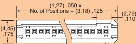
SINGLE ROW
