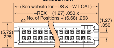
DOUBLE ROW
