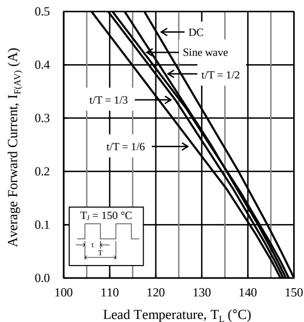
Figure 3. Typical Characteristics: I_{F(AV)} vs. T_L^{(2)} ( V_R = 800 V)
