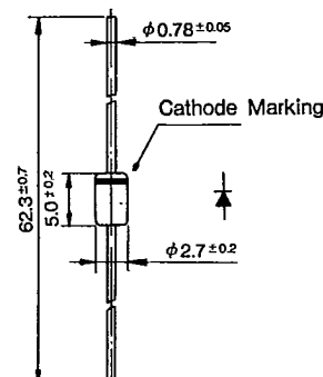
Outline Drawing ③⑦
