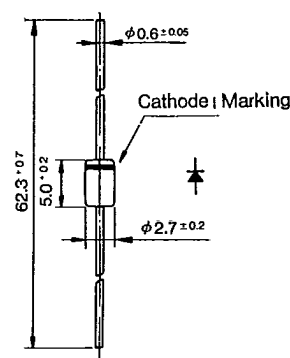
Outline Drawing ③⑤
