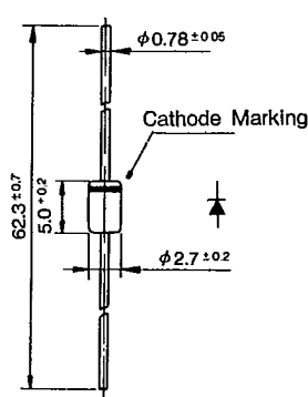
Outline Drawing ③④
