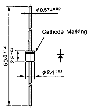
Outline Drawing ③⑥
