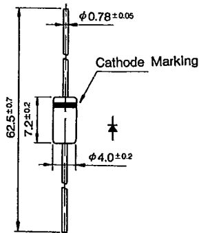
Outline Drawing ③⑥
