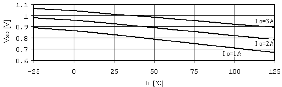
SLA7062M/67M
