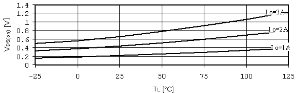
SLA7062M/67M
