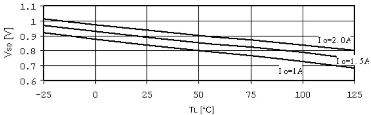
SLA7062M/67M
