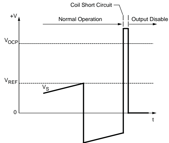
Figure 4. Motor coil short circuit protect circuit operation. Overcurrent that flows without passing the sense resistor is undetectable. To recover the circuit after protection operates, VDD must be cycled and started up again.
