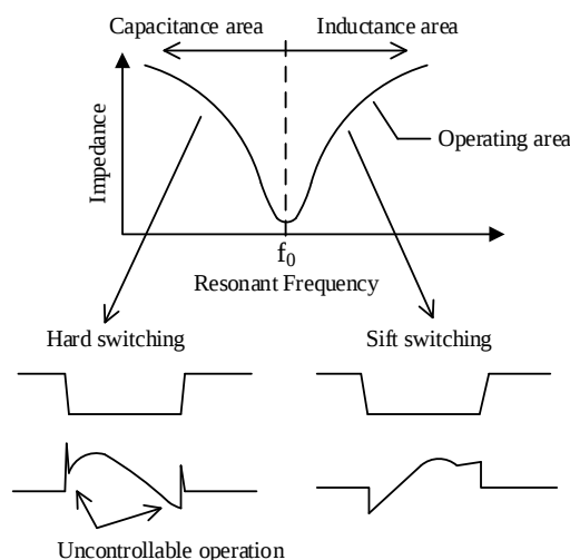
Figure 8-30. Operating Area of Resonant Power Supply
