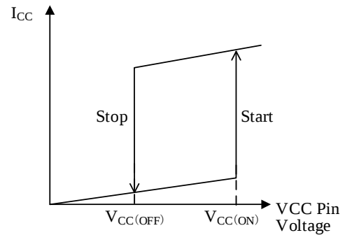
Figure 8-15. V_{CC} vs. I_{CC}
