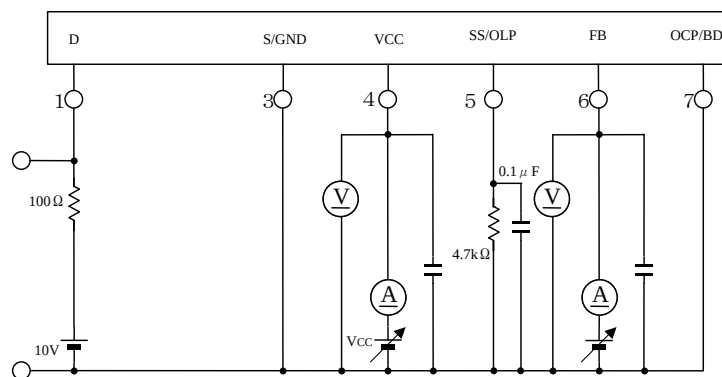
Measurement Circuit 4
