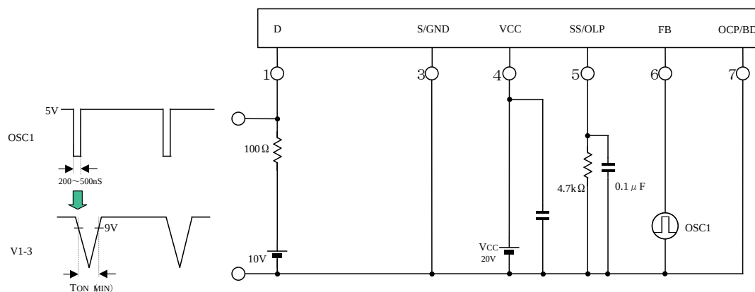
Measurement Circuit 6
