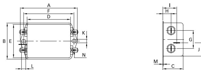
Connection style -06, 16 and 20A types
