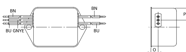
Connection style -07, 16 and 20A types (same dimensions as style -06)
