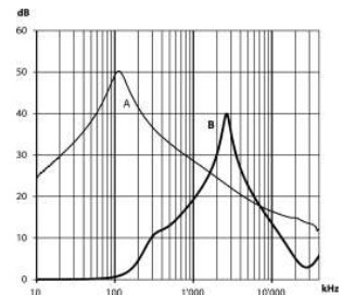
2'300A types
