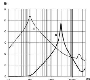
600 A types
