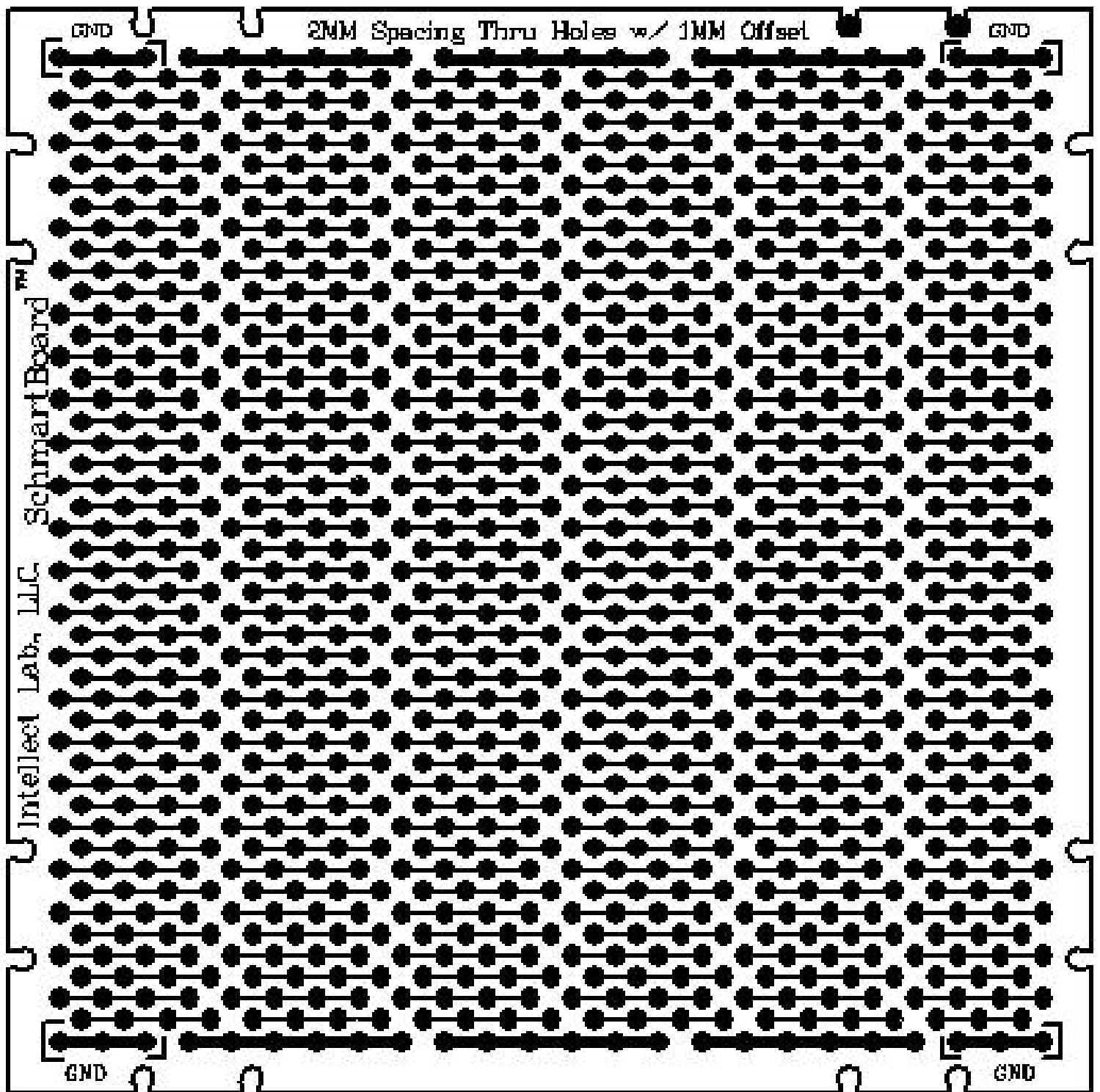
2mm Spacing With 1mm Offset (201-0002-01) Top Side
