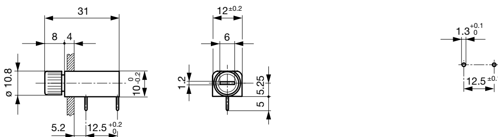
Drilling diagram
