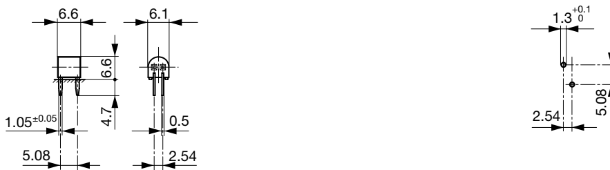
Drilling diagram
