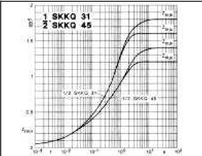
Fig. 3 Thermal transient impedance vs. time
