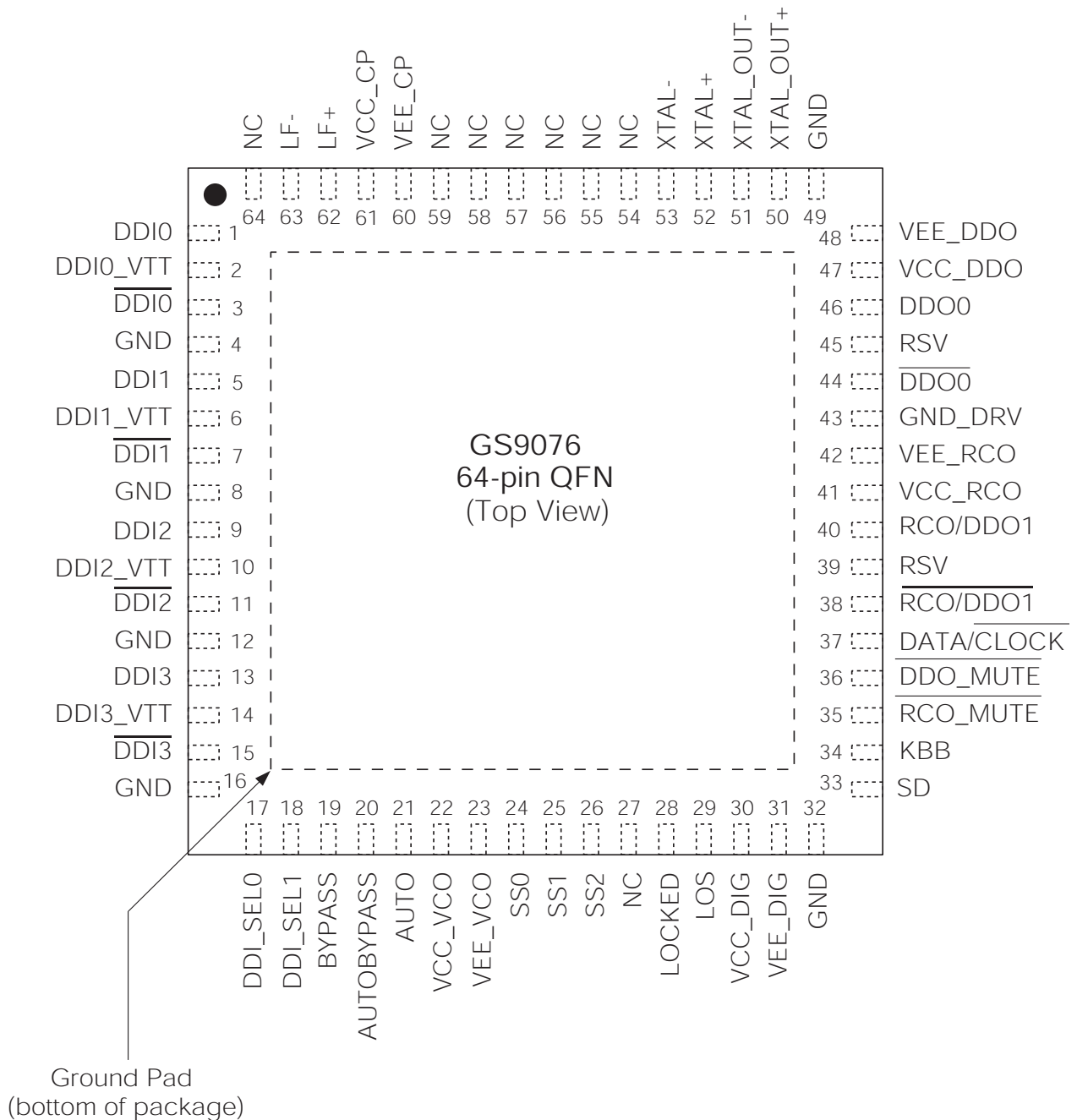
Figure 1-1: 64-Pin QFN
