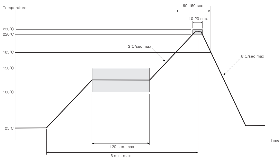
Figure 2-4: Standard Pb Solder Reflow Profile
