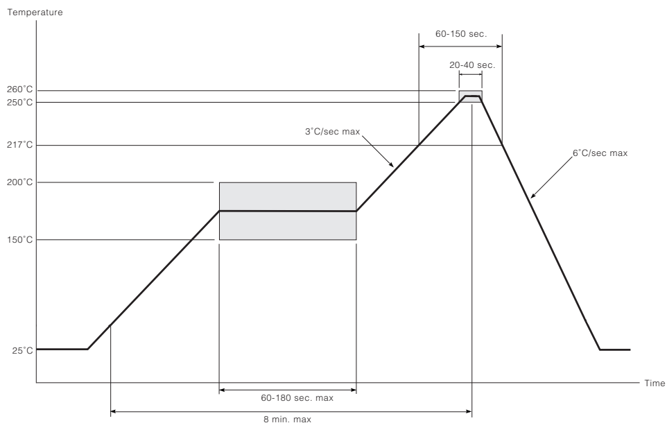
Figure 2-3: Maximum Pb-free Solder Reflow Profile (Preferred)
