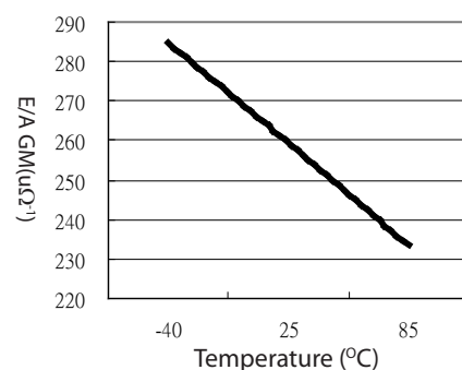
E/A GM vs. Temperature
