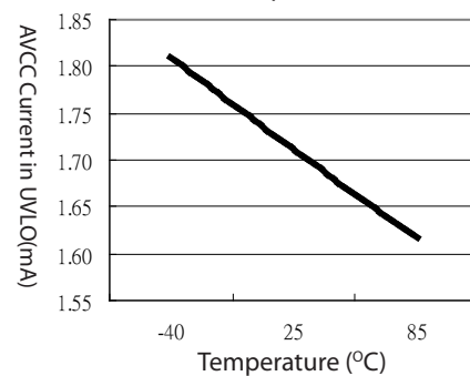
AVCC current in UVLO vs. Temperature
