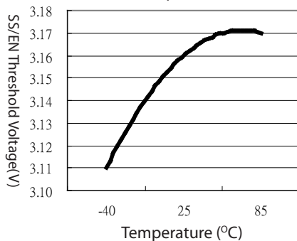
SS/EN Threshold for Overload Hiccup vs. Temperature
