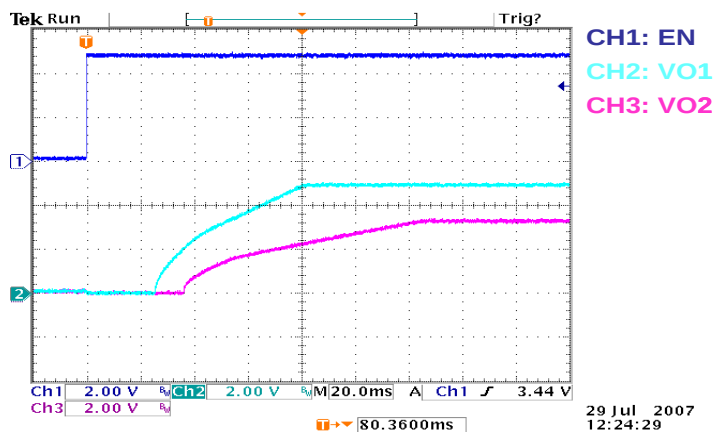
Ratiometric start up(connect SS1,SS2 together).
