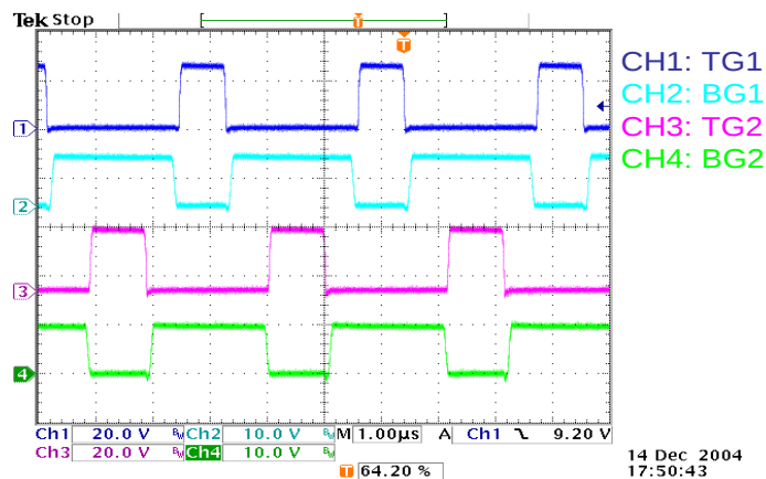
Gate waveform
