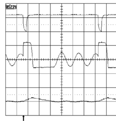
Buck-Boost DCM Operation
