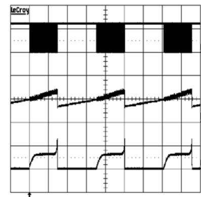
Buck Overcurrent Protection
