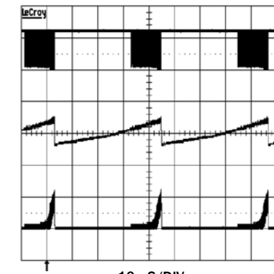
Buck-Boost Overcurrent Protection
