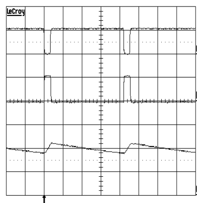
Buck CCM Operation
