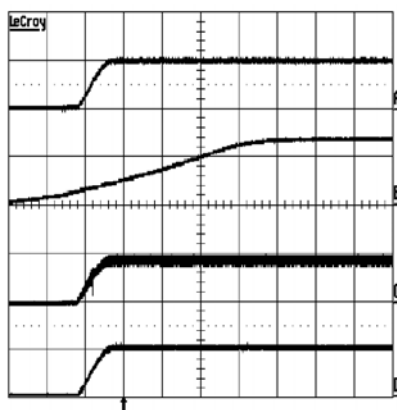
Buck Converter Sartup
