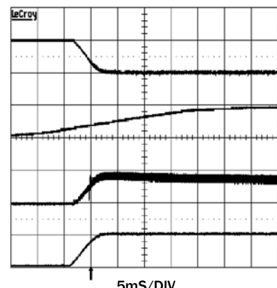
Buck-Boost Converter Startup
