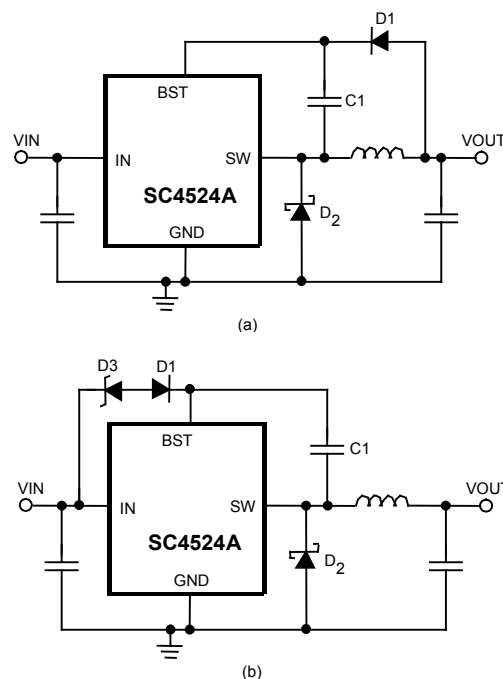
Figure 6. Methods of Bootstrapping the SC4524A
