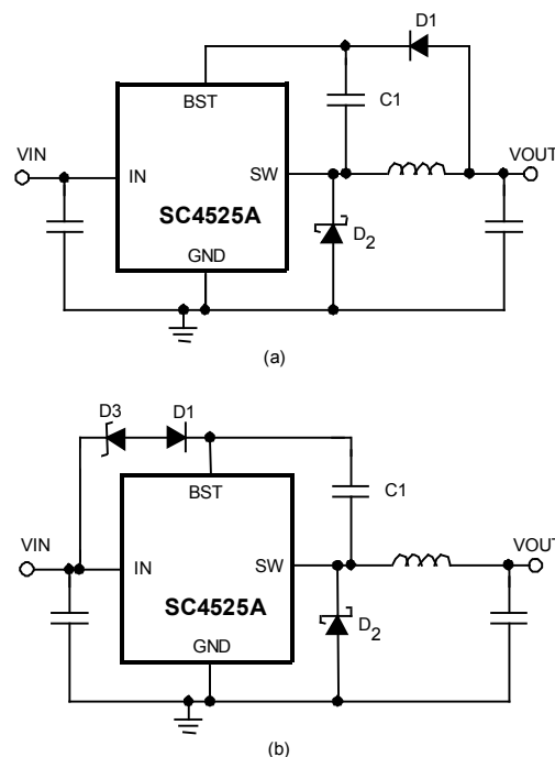
Figure 6. Methods of Bootstrapping the SC4525A
