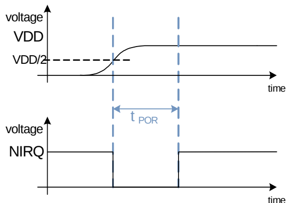
Figure 28. Power-up, NIRQ
