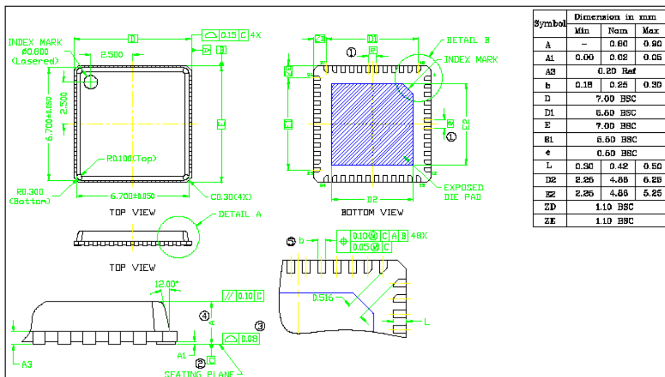
Figure 25: Package Dimensions
