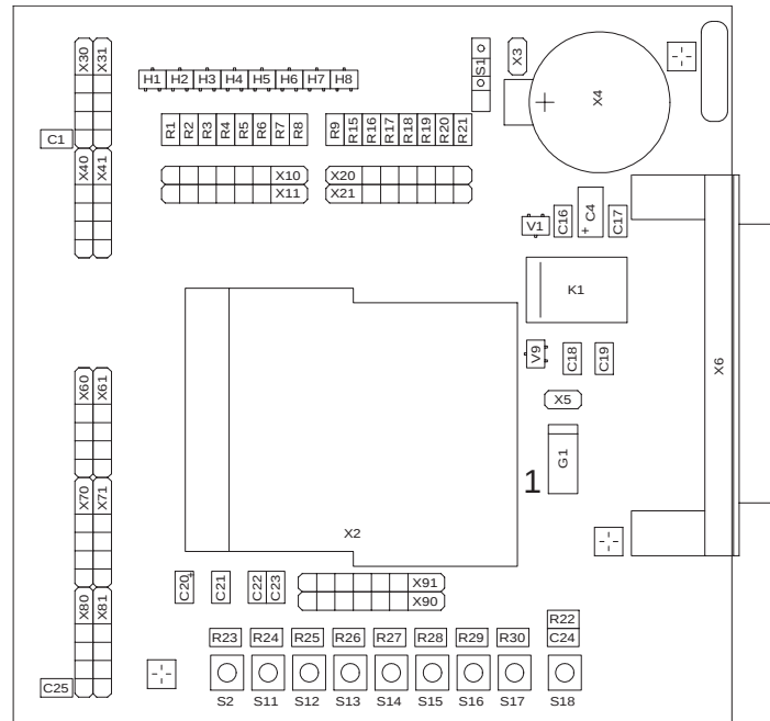
Figure 2 : XE8000EV101 implantation map
