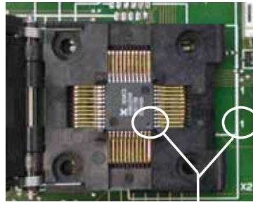
pin 1 markers
