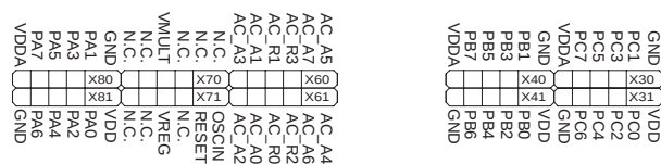
Figure 2 : XE8000EV101 implantation map
