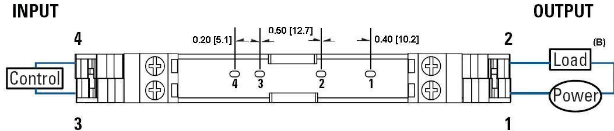
Wiring Diagram (A)
