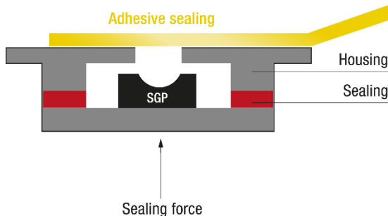
Figure 9 Cover the device cavity where the SGPxx is located by a recommended adhesive during shipment until final use as well as during rework and repair.
