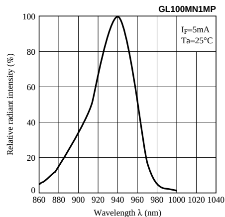
Fig.4 Spectral Distribution
