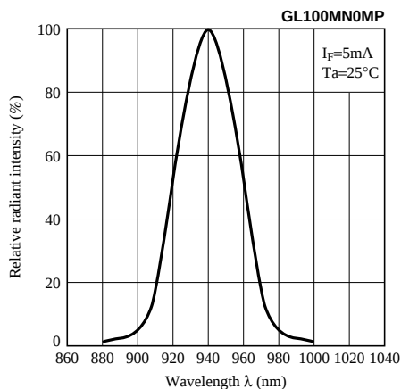
Fig.3 Spectral Distribution
