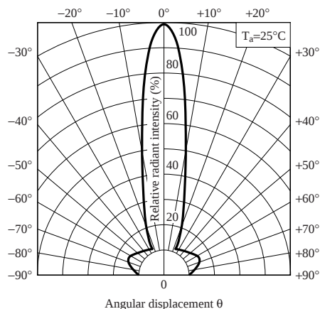
Fig.14 Radiation Diagram (Typical Value)
