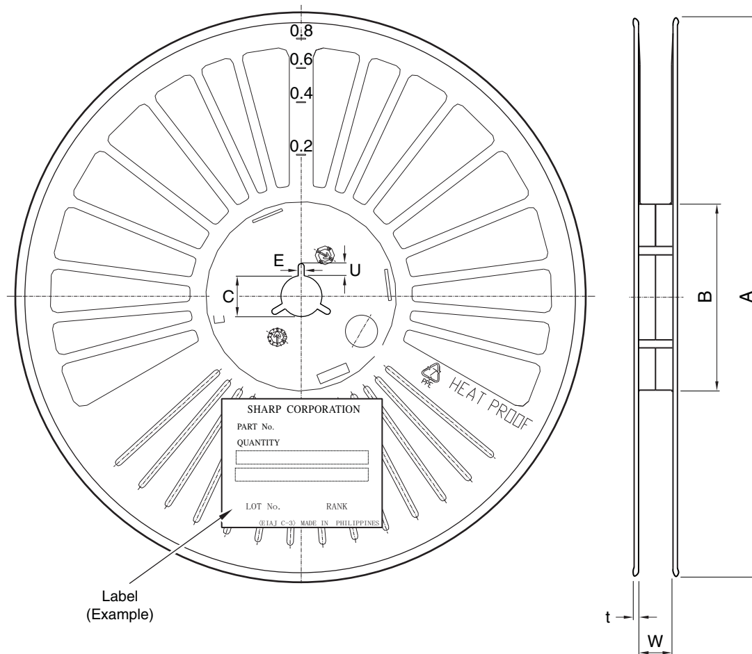
Fig. 11 Reel Shape and Dimensions
