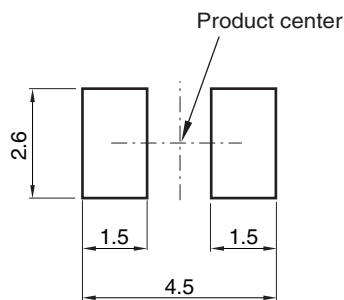
Fig. 17 Recommended Solder Pad Design
