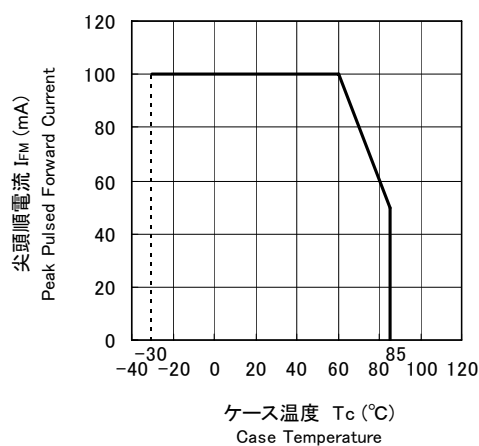
尖頭順電流低減曲線 Peak Pulsed Forward Current Derating Curve
