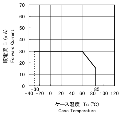
順電流低減曲線 Forward Current Derating Curve
