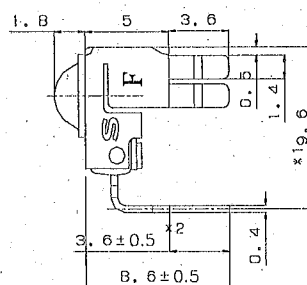
Example of mounting drawing from solder side(Reference)
