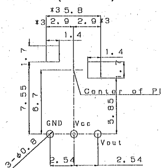
Example of mounting drawing from solder side(Reference)
