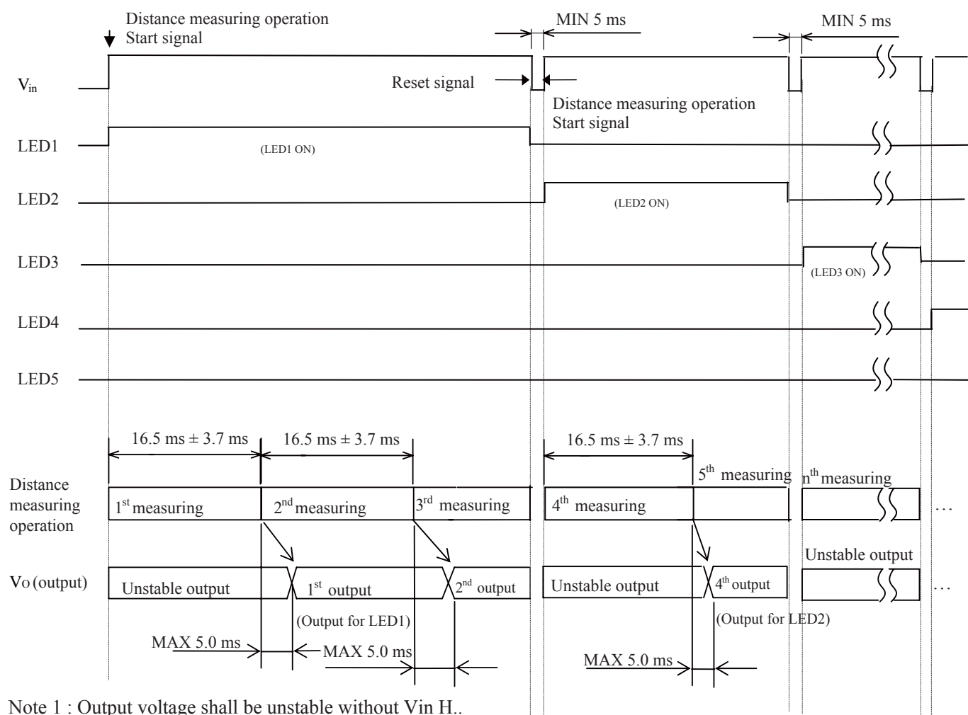
Fig. 1 Timing chart
