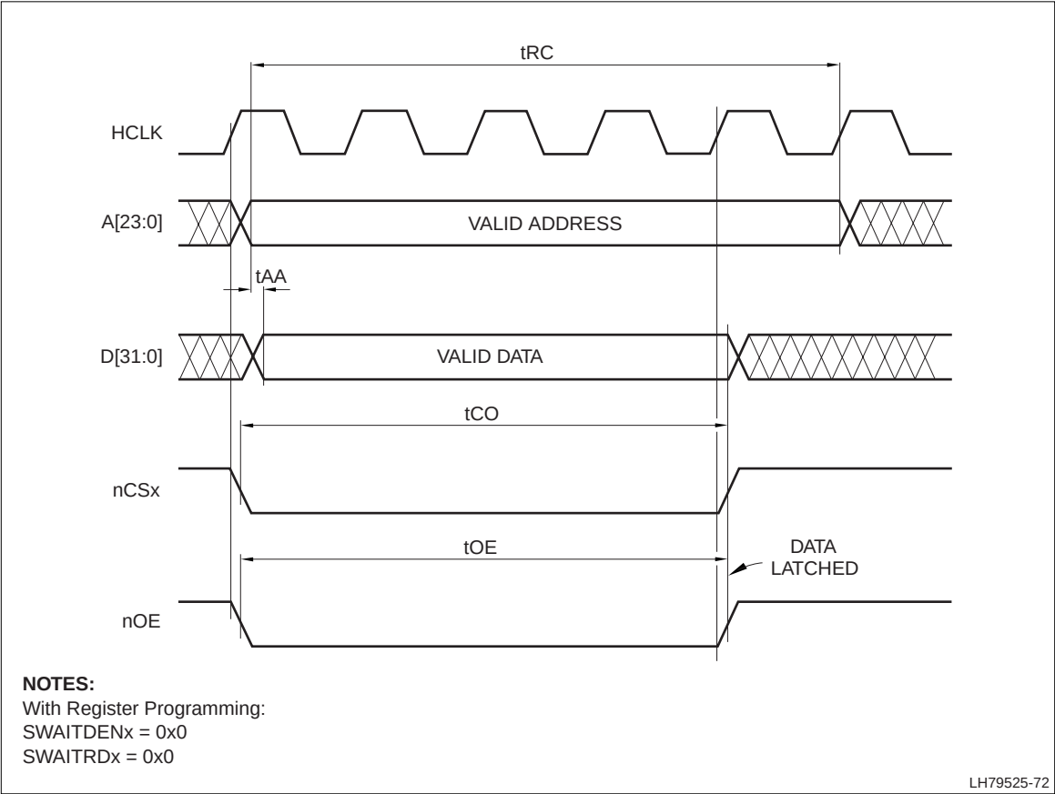
Figure 12. External Static Memory Read with Three Wait States
