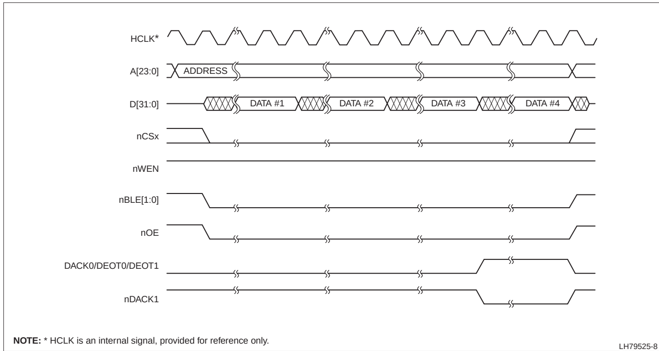
Figure 19. Read, Peripheral to Memory: Peripheral Burst Size = 4
