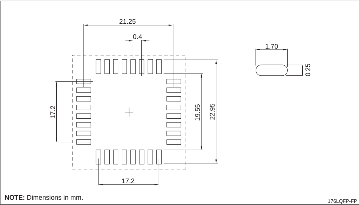
Figure 36. LH79525: 176-pin LQFP PCB Footprint
