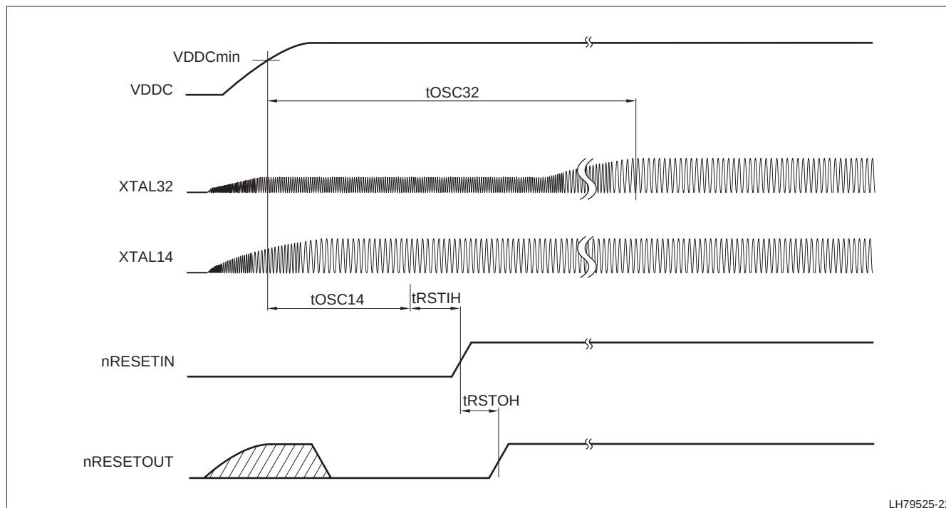
Figure 30. PLL Start-up
