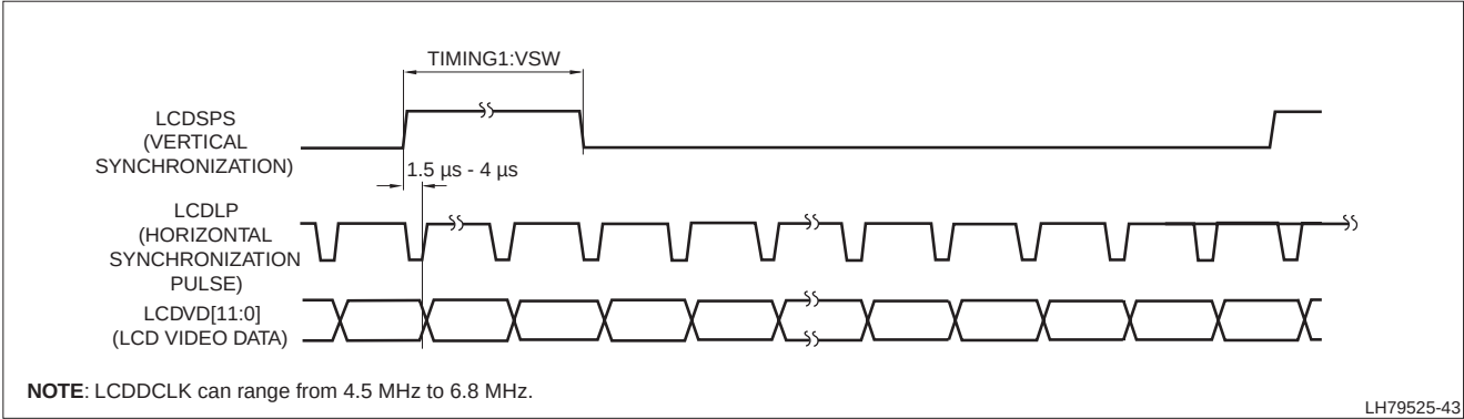
Figure 26. AD-TFT, HR-TFT Vertical Timing
