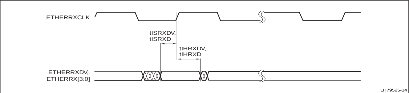
Figure 29. Ethernet Receive Timing
