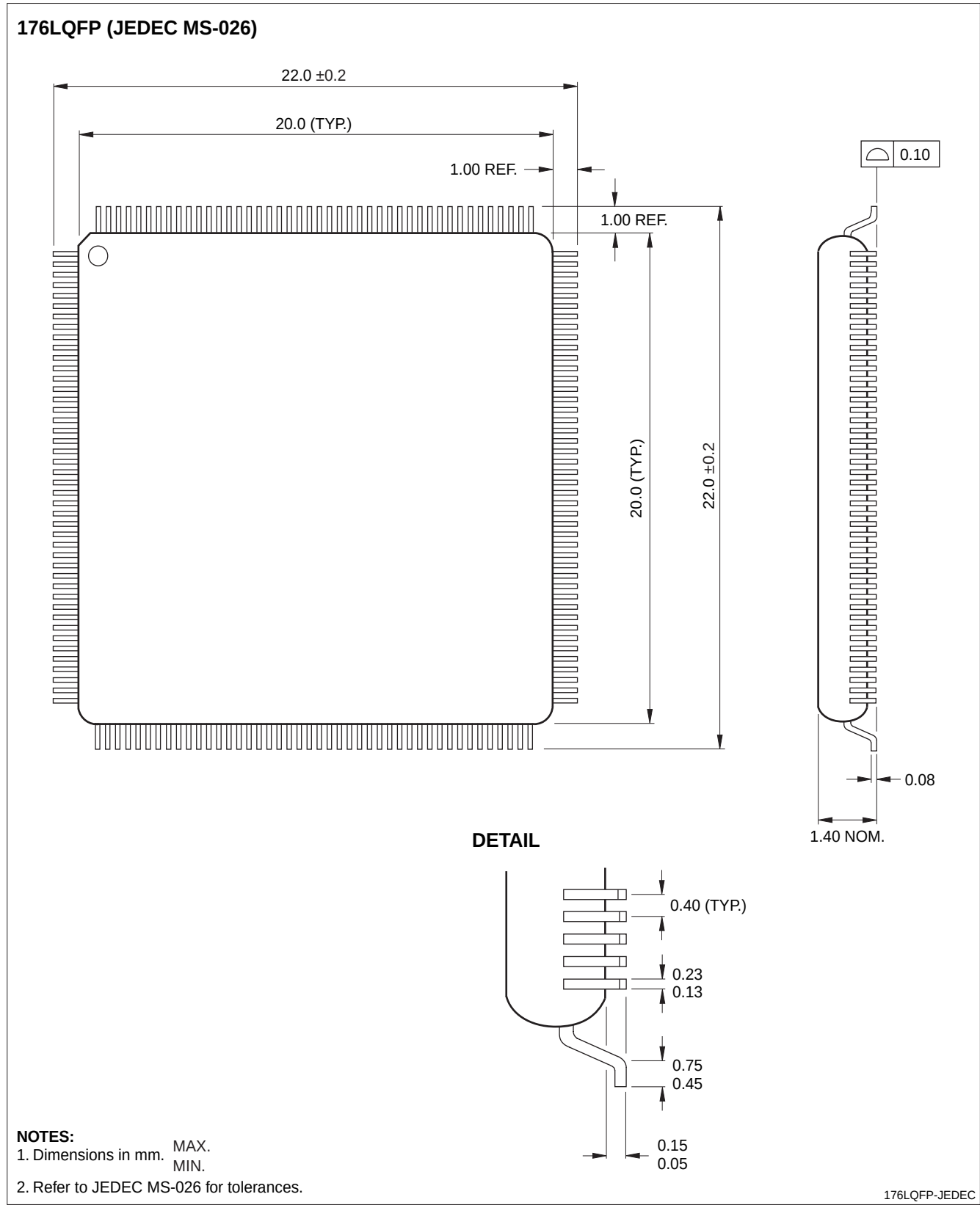
Figure 34. LH79525: 176-pin LQFP
