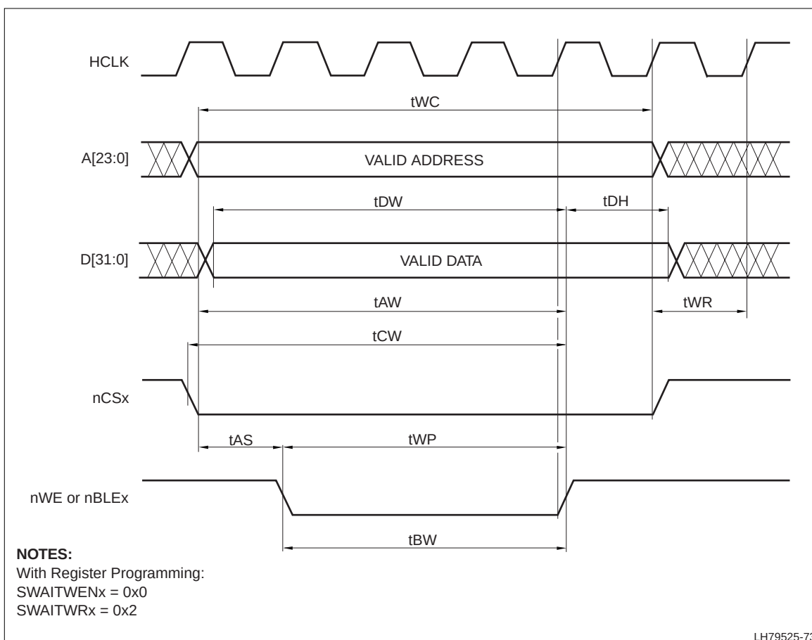
Figure 13. External Static Memory Write with Two Wait States
