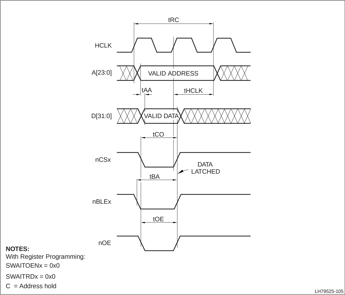
Figure 10. External Static Memory Read, Zero Wait States
