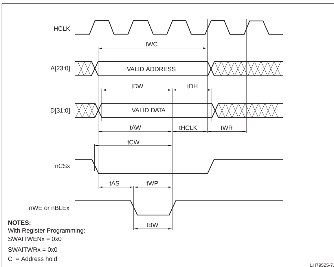
Figure 11. External Static Memory Write, Zero Wait States
