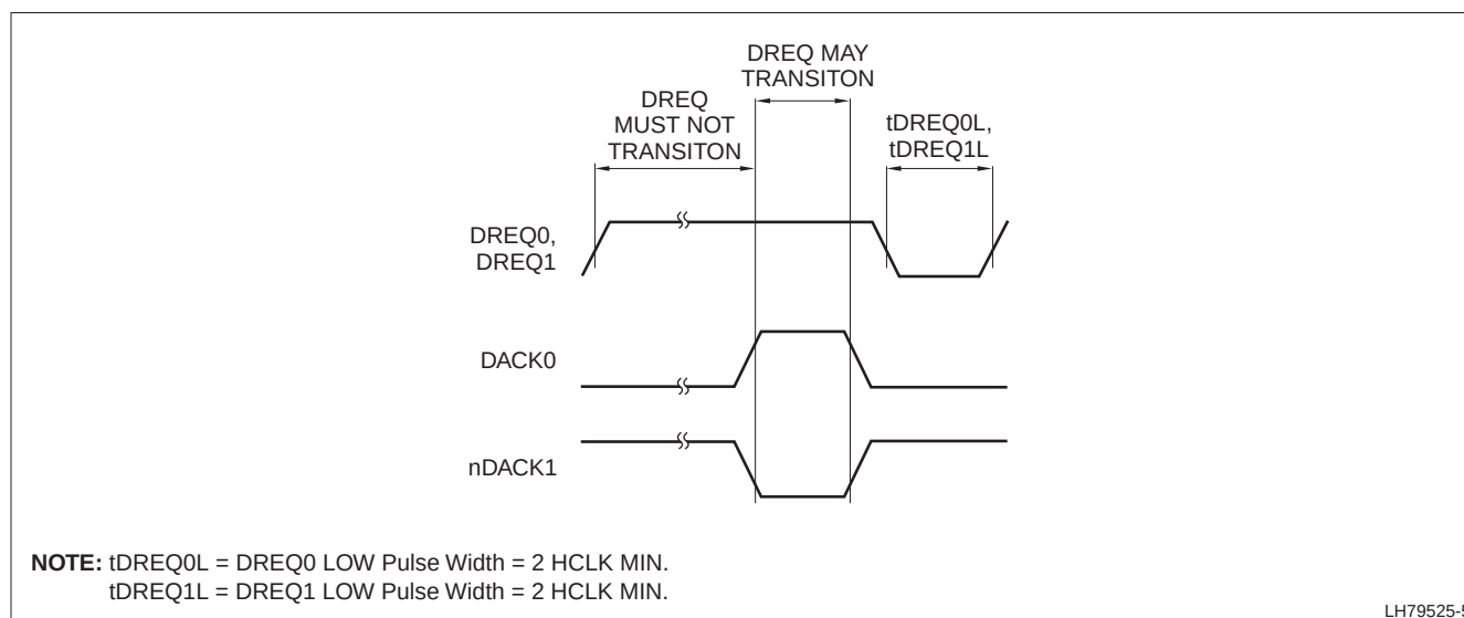
Figure 16. DREQ Timing Restrictions
