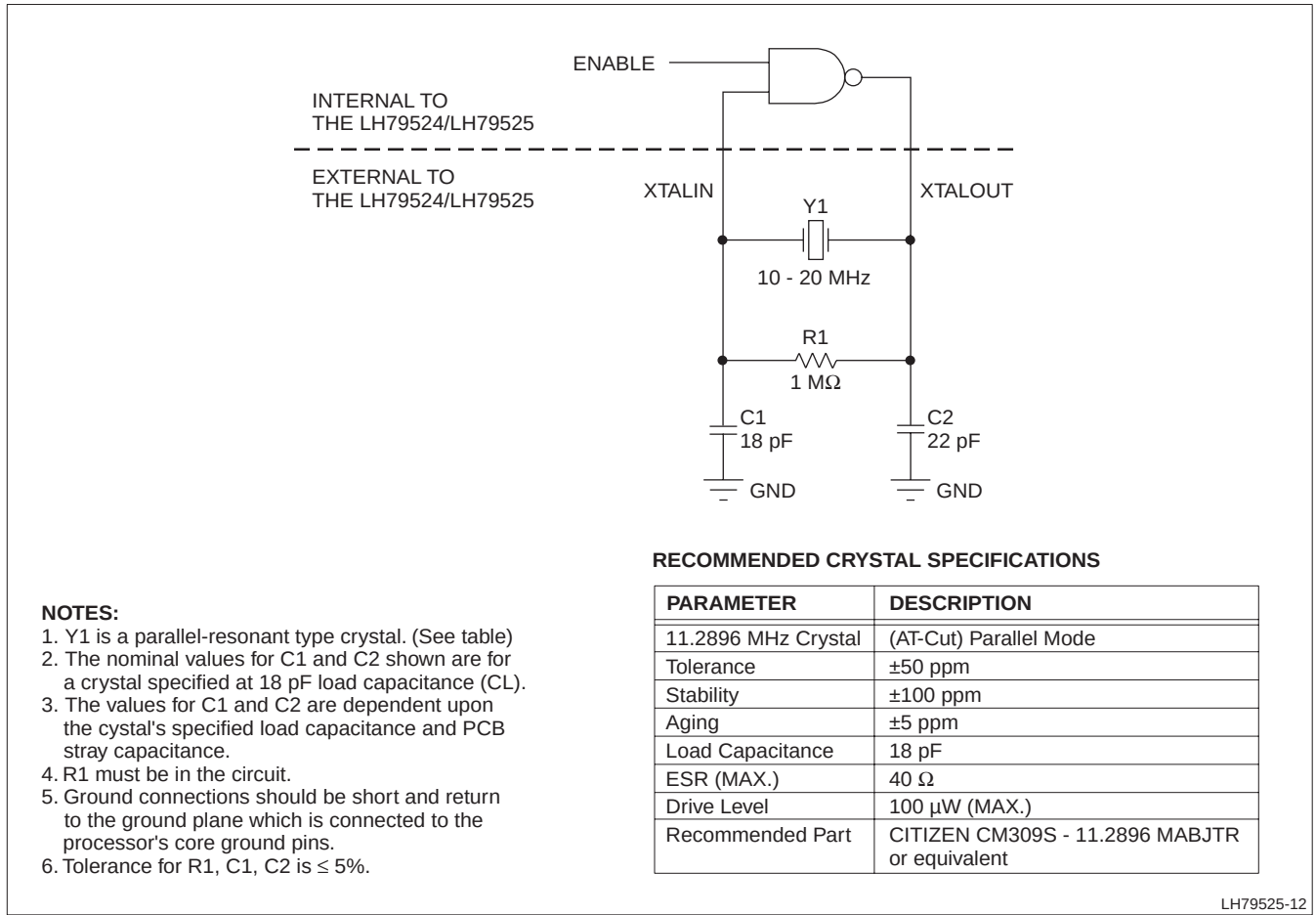
Figure 33. Suggested External Components, 10 - 20 MHz Oscillator
