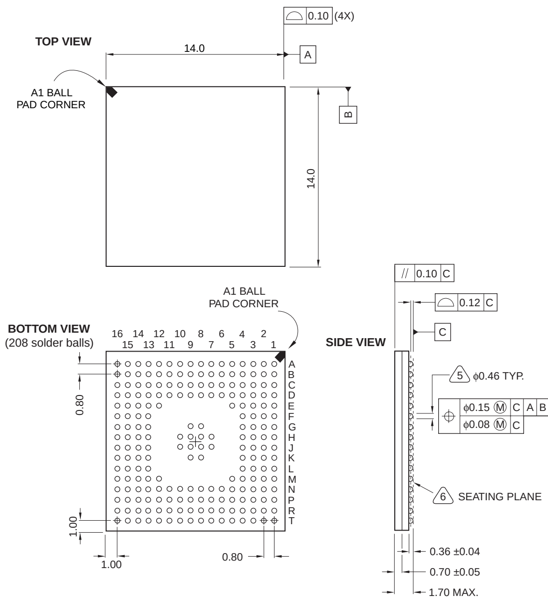
Figure 35. LH79524: 208-ball CABGA
