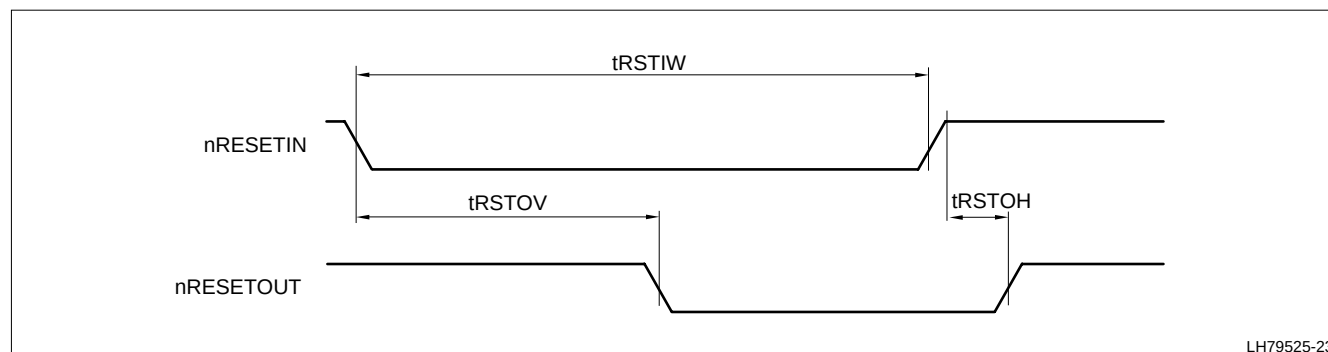
Figure 31. External Reset
