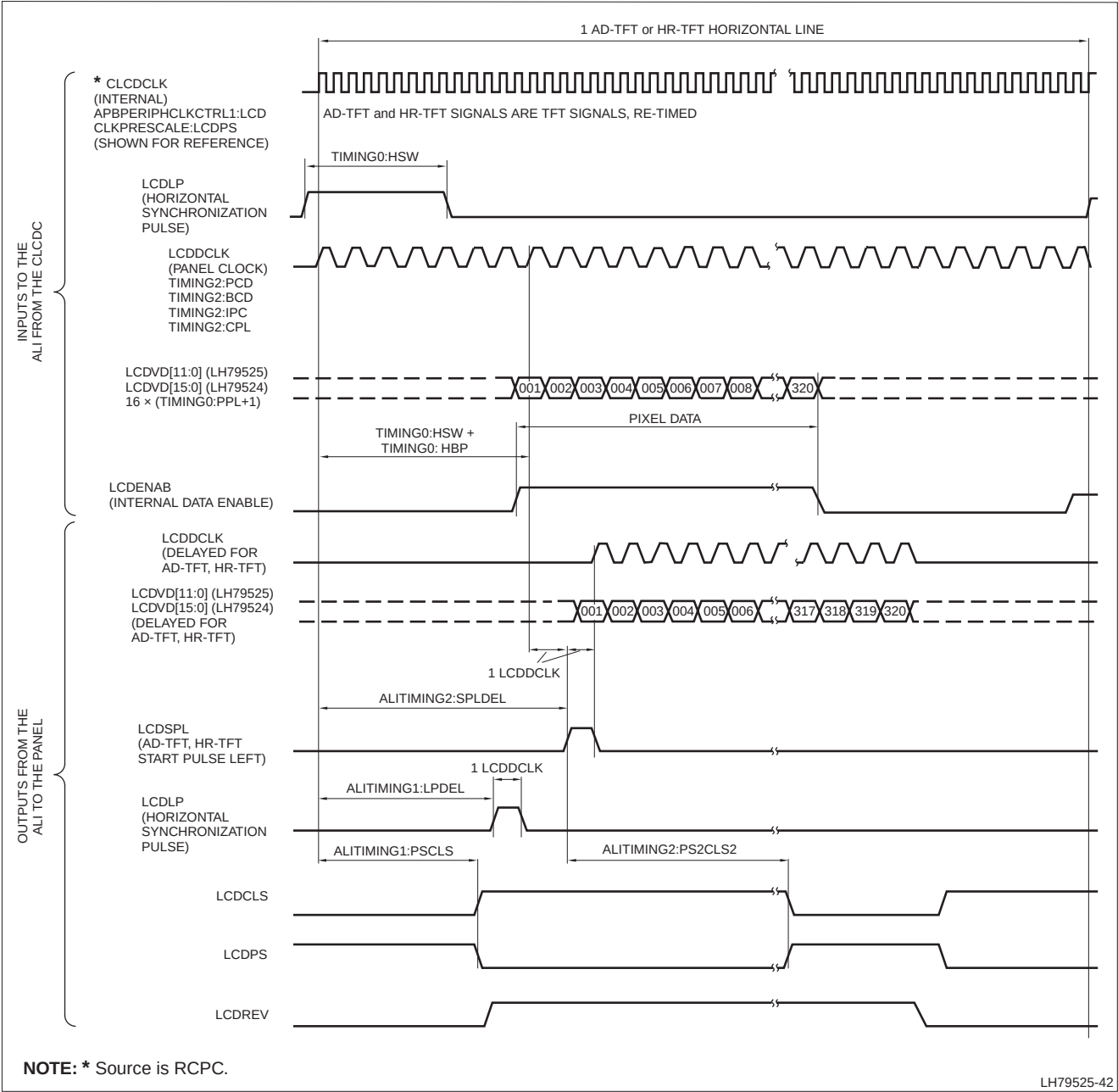
Figure 25. AD-TFT, HR-TFT Horizontal Timing
