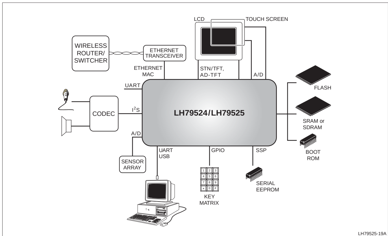
Figure 2. LH79524/LH79525 Application Diagram Example
