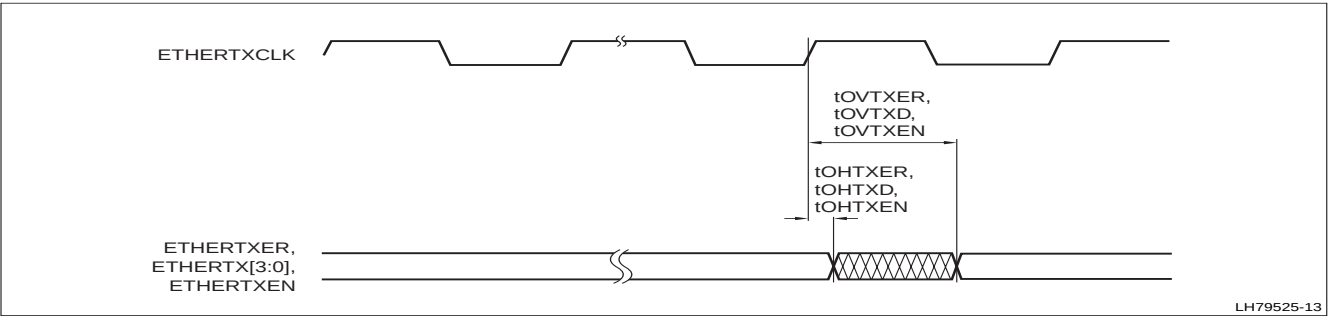
Figure 28. Ethernet Transmit Timing
