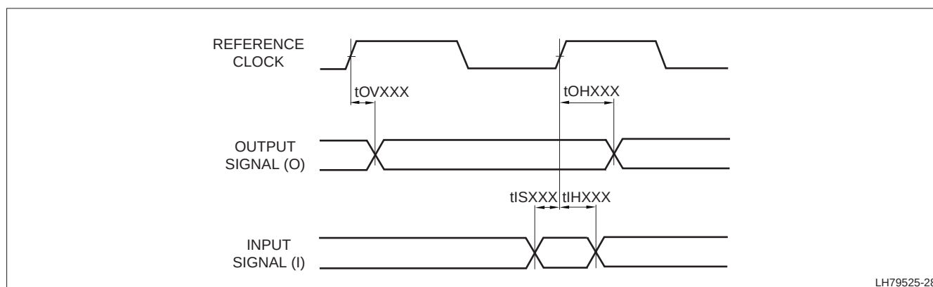
Figure 7. LH79524/LH79525 Signal Timing
