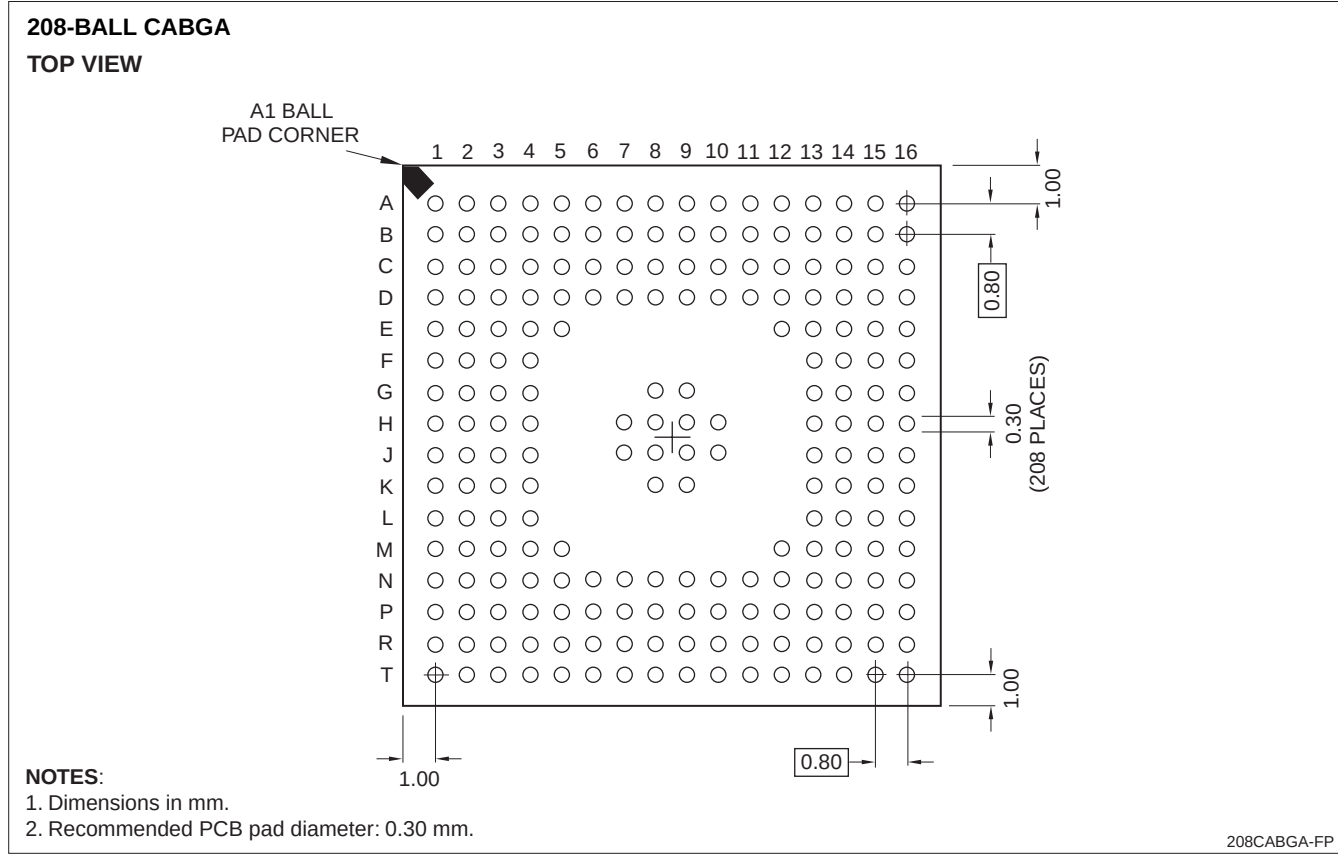
Figure 37. LH79524: 208-ball CABGA PCB Footprint
