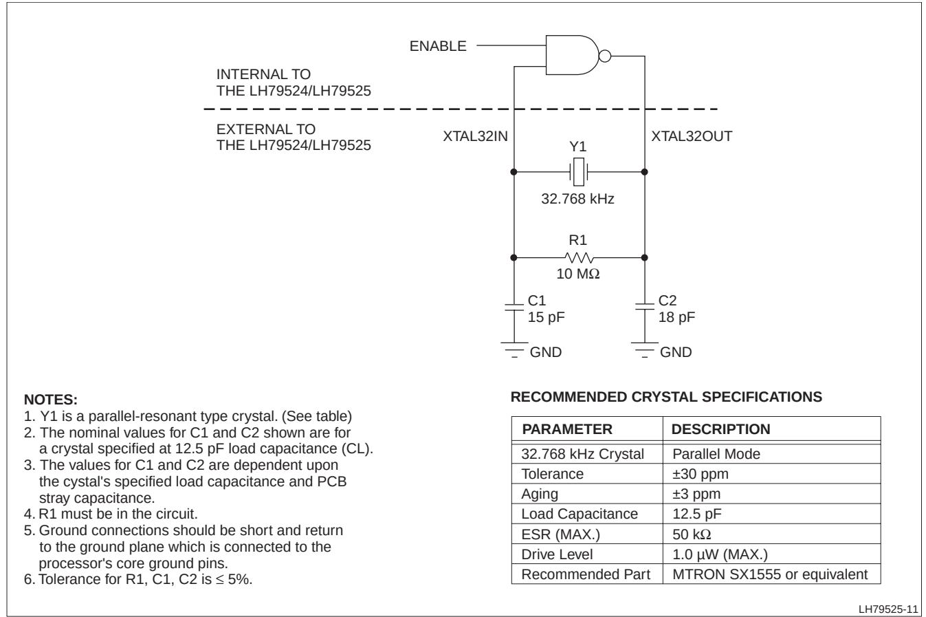
Figure 32. Suggested External Components, 32.768 kHz Oscillator (XTAL32IN and XTAL32OUT)
