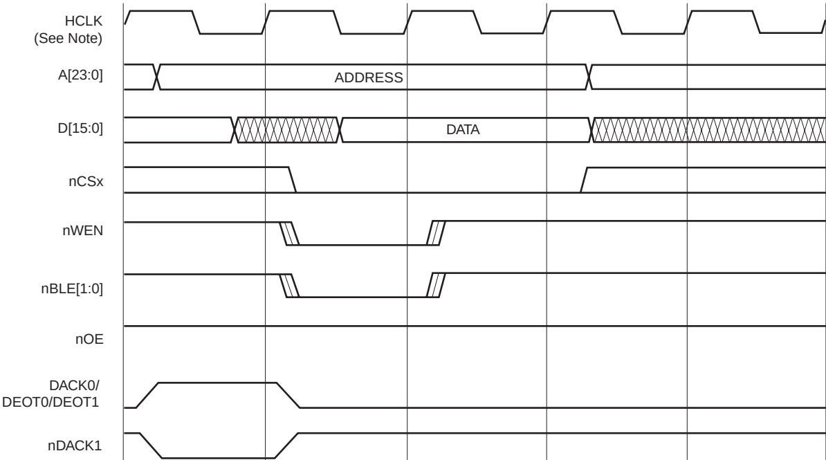
Figure 18. Write, from Memory to Peripheral, Burst Size = 1
