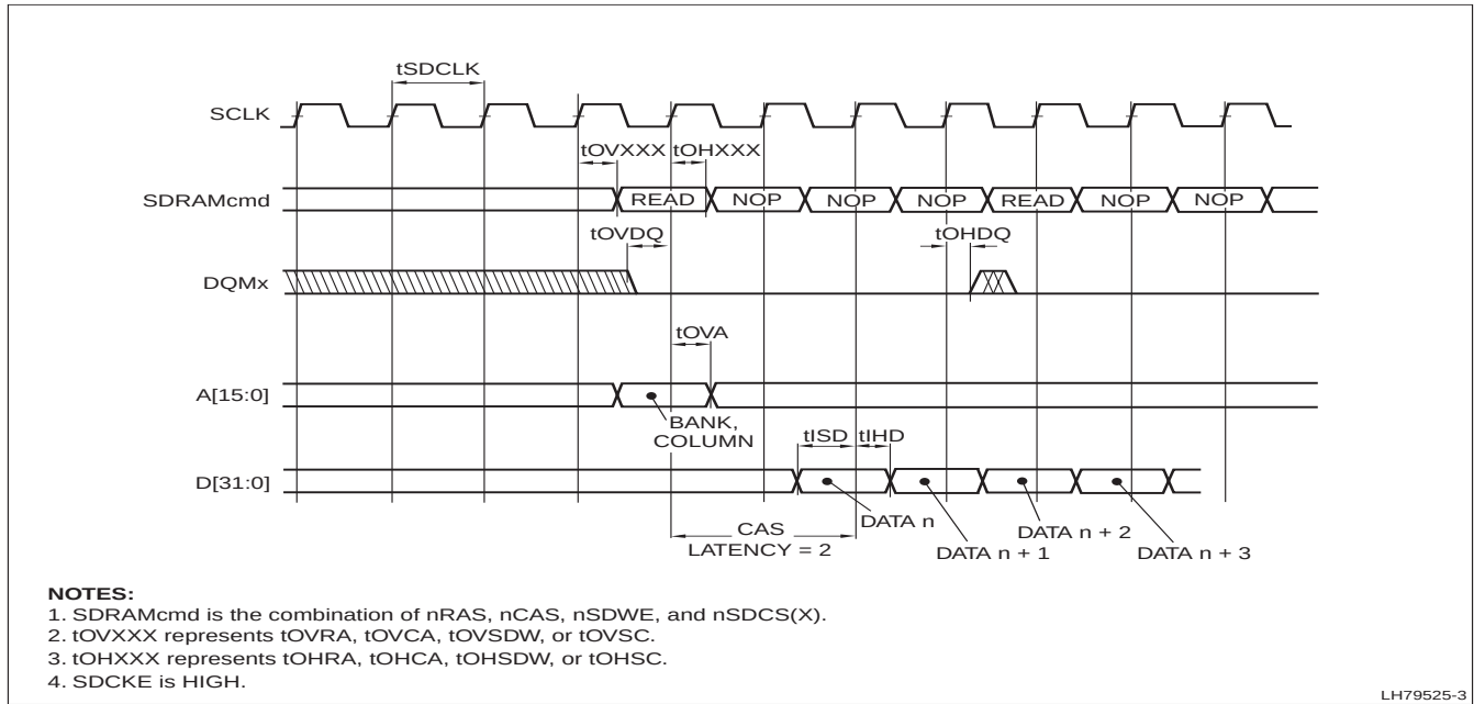
Figure 14. SDRAM Burst Read
