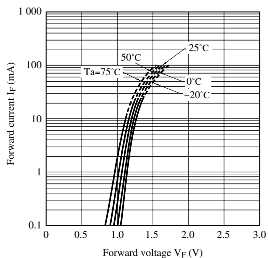
Fig.10 Forward Current vs. Forward Voltage
