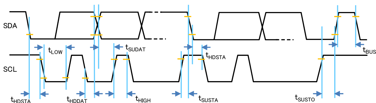
I 2 C Timing Diagram
