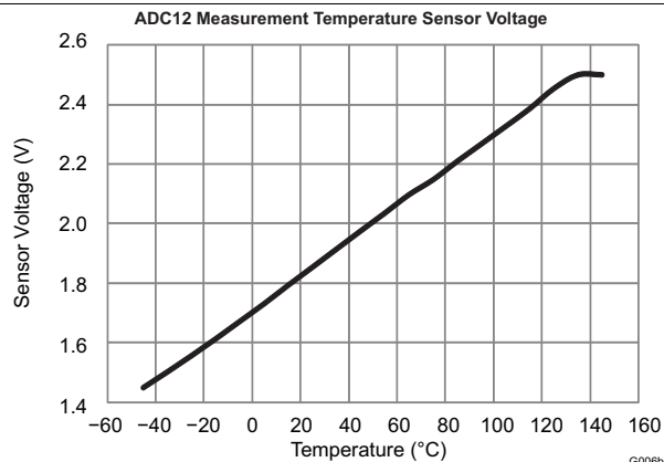
Figure 5-6. ADC12 Measurement Temperature Sensor Voltage vs Temperature
