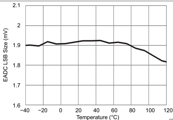
Figure 5-5. EADC LSB Size with 4X Gain (mV) vs Temperature
