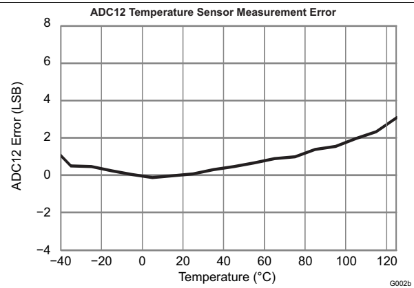
Figure 5-8. ADC12 Temperature Sensor Measurement Error vs Temperature
