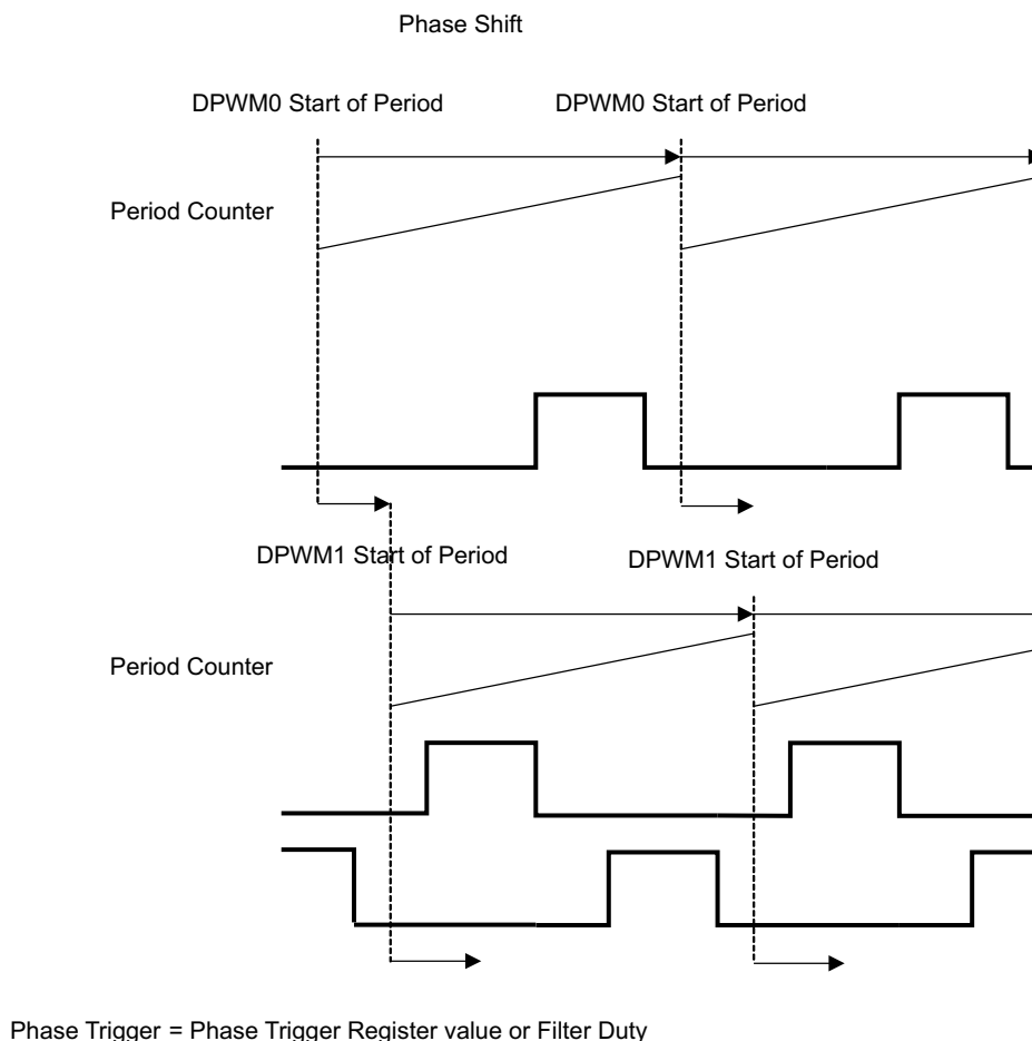
Figure 6-23. Phase Shifting
