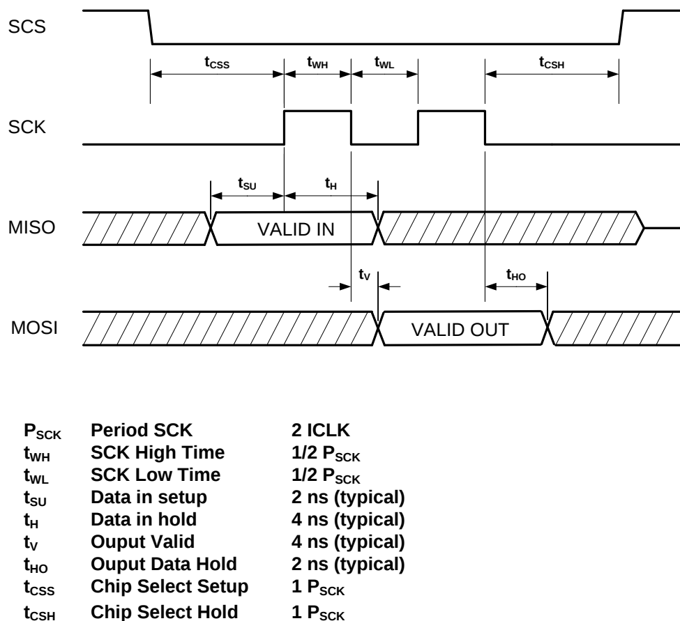
Figure 6-18. SPI Timing Diagram
