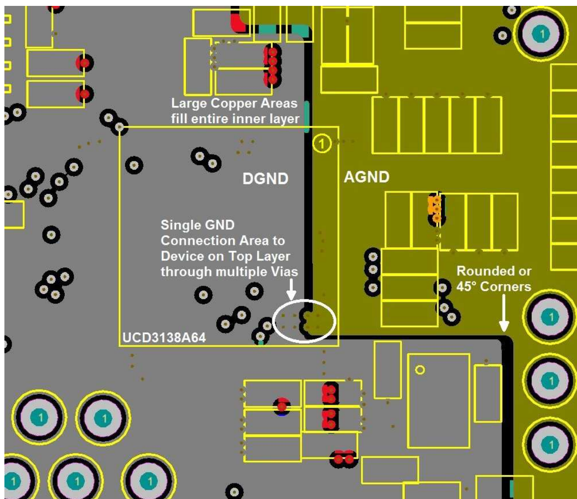
Figure 7-13. Layout Example
