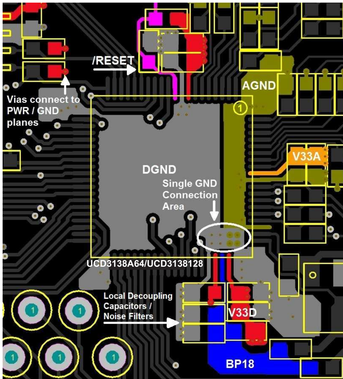
Figure 7-14. Layout Example
