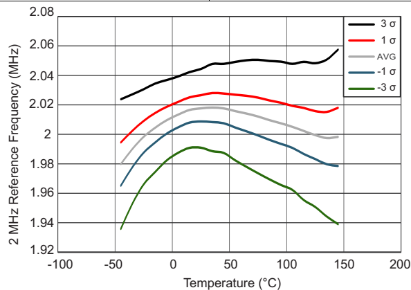
Figure 5-9. Oscillator Frequency (2MHz Reference, Divided Down from 250MHz) vs Temperature
