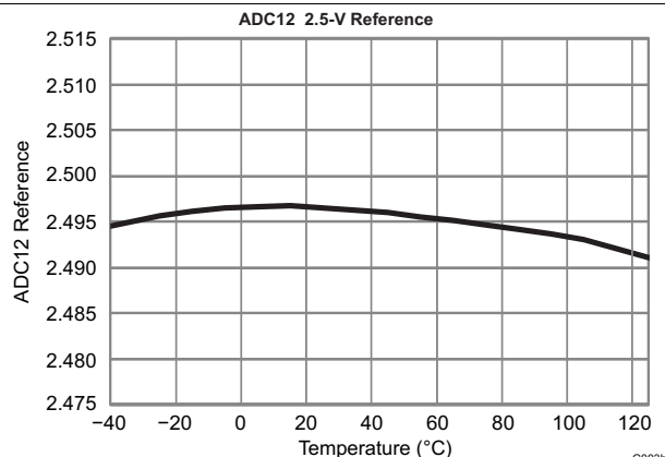
Figure 5-7. ADC12 2.5-V Reference vs Temperature
