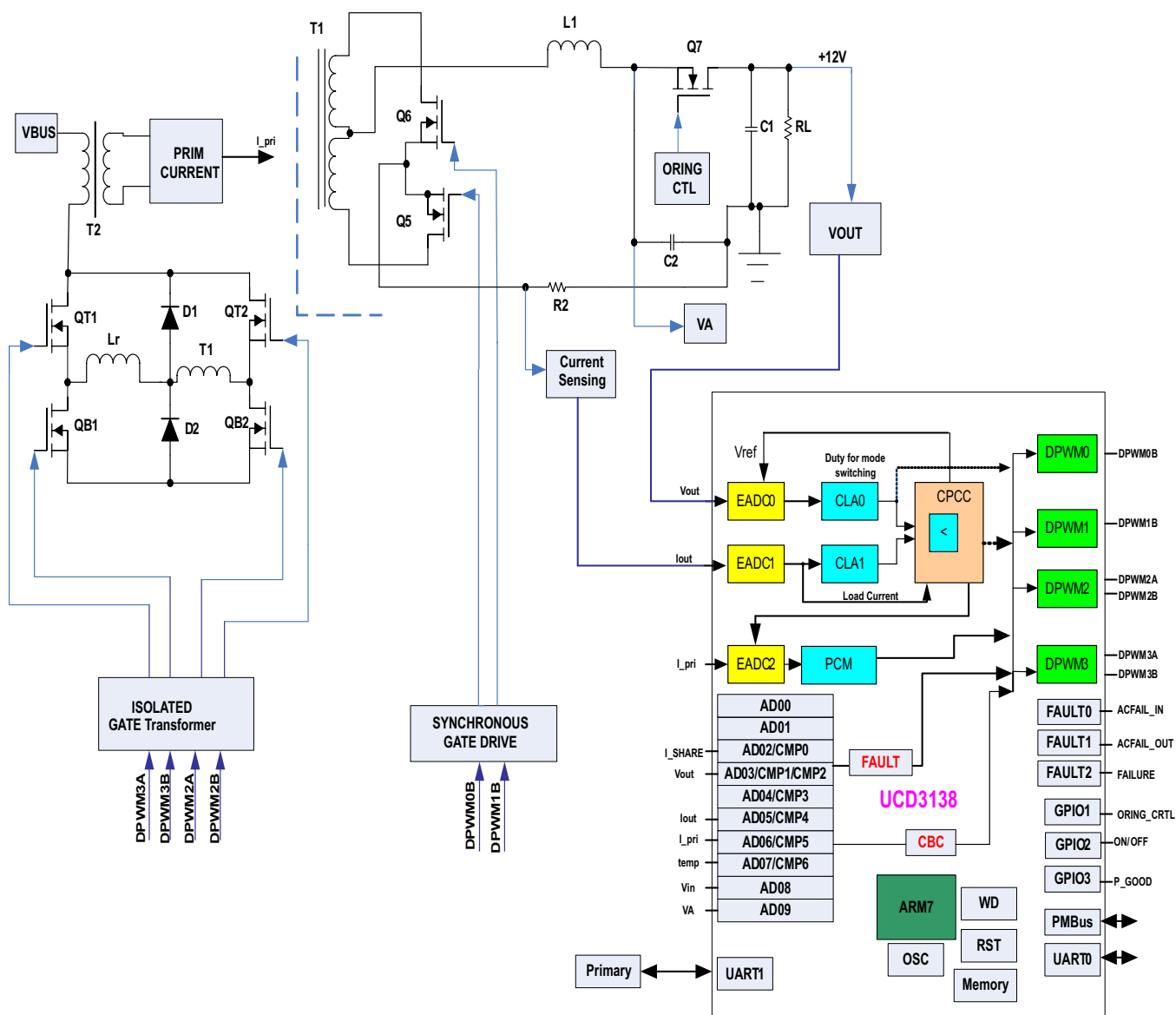
Figure 7-1. Phase-Shifted Full-Bridge
