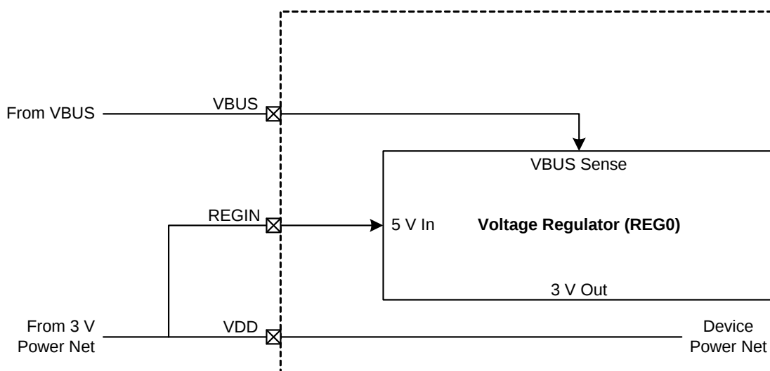
Figure 8.3. REG0 Configuration: USB Self-Powered, Regulator Disabled
