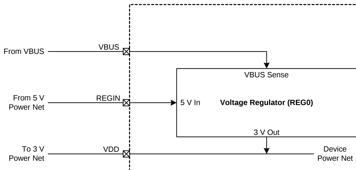
Figure 8.2. REG0 Configuration: USB Self-Powered
