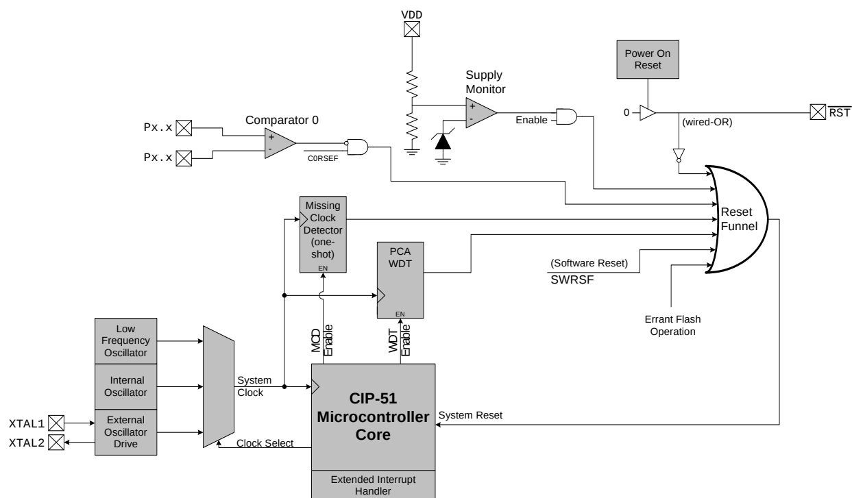
Figure 16.1. Reset Sources
