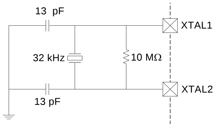
Figure 18.2. External Crystal Example
