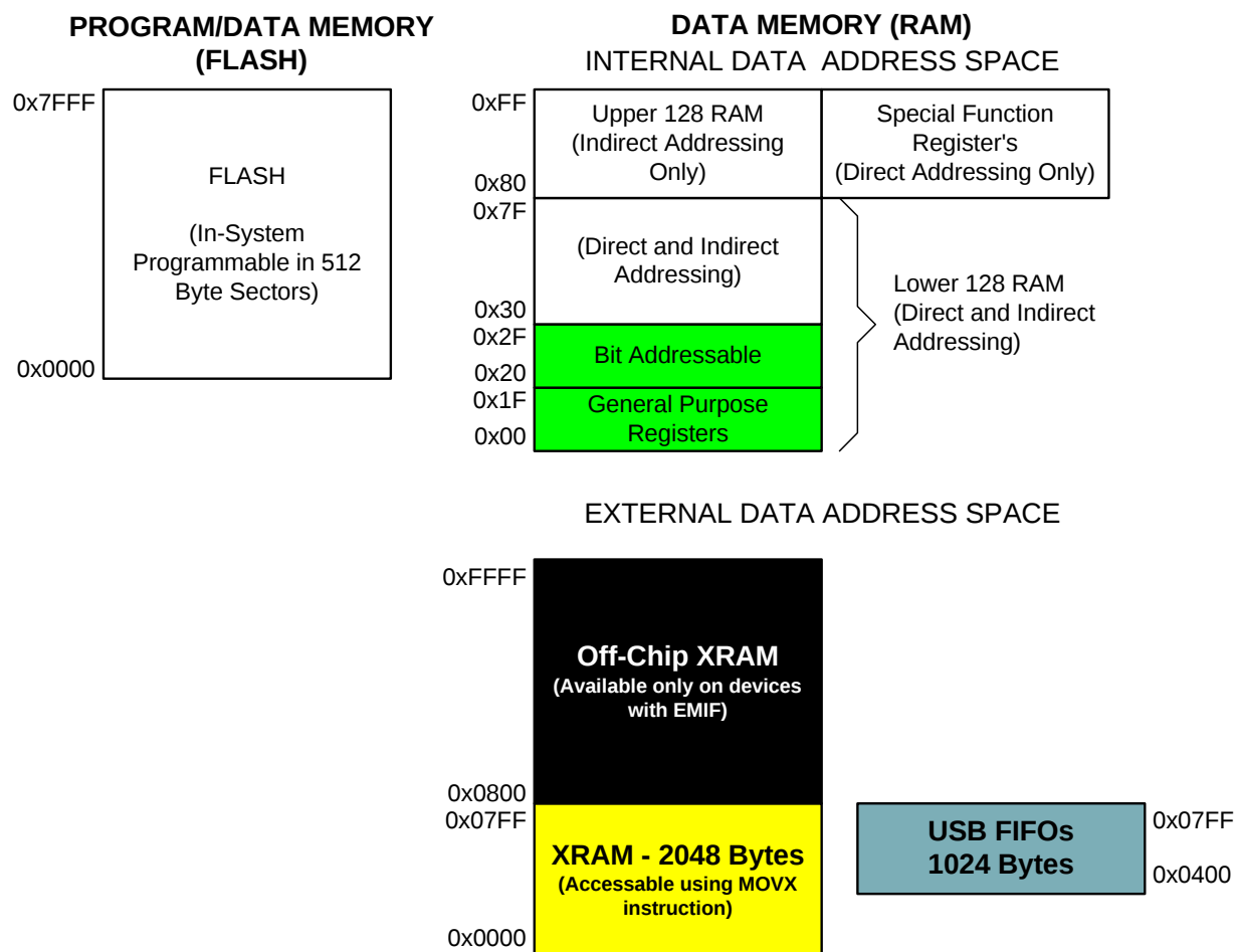
Figure 12.2. On-Chip Memory Map for 32 kB Devices (C8051F382/3/6/7)
