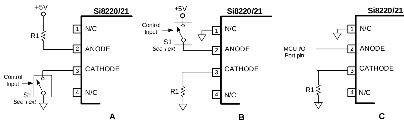
Figure 15. Si8220/21 Other Input Circuit Configurations
