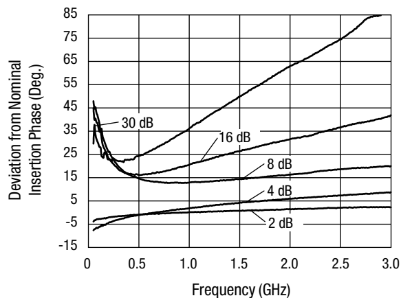
Attenuation Phase Accuracy vs. Frequency (85 °C)
