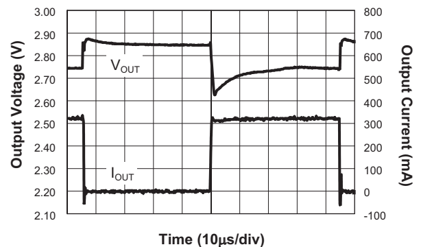
Over-Current Protection
