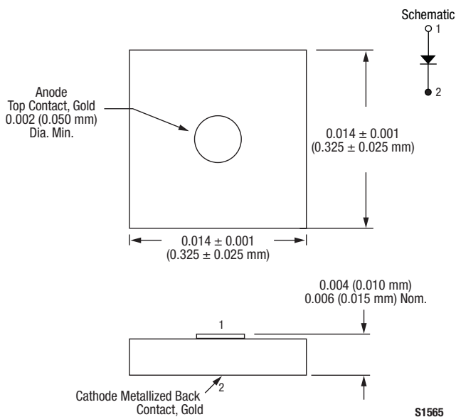
Figure 3. 149-815 Package
