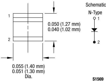
Figure 5. -203 Package
