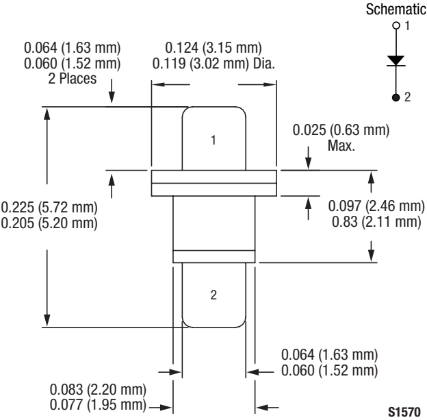
Figure 6. -210 Package
