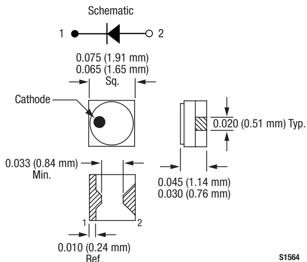
Figure 7. -219 Package
