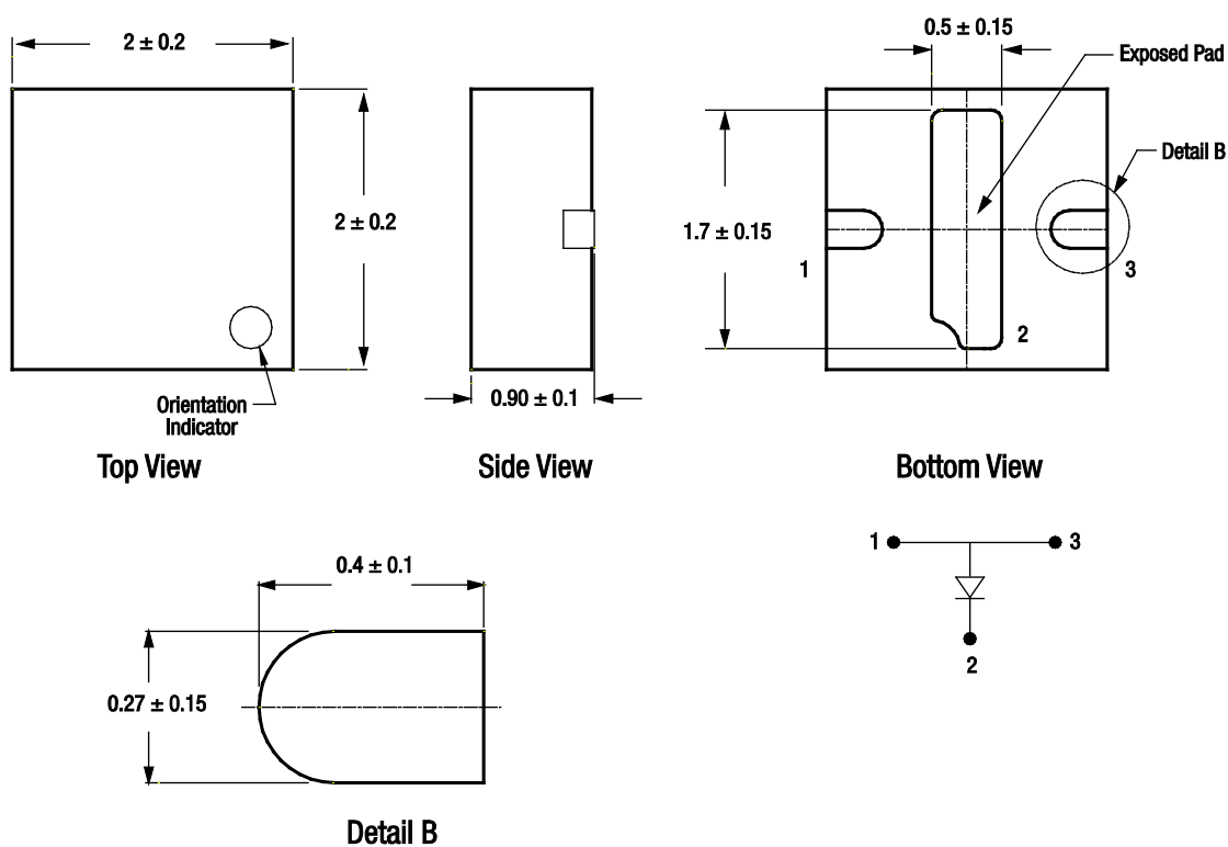
Figure 10. CLA4608-085LF QFN Package Dimension Drawing
