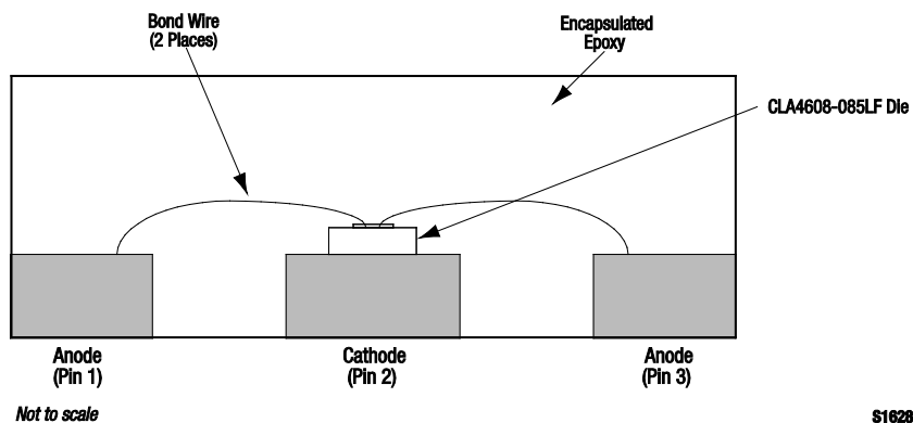
Figure 6. Cross-Sectional View of the CLA4608-085LF
