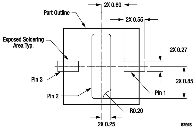
Figure 8. CLA4608-085LF PCB Layout Footprint
