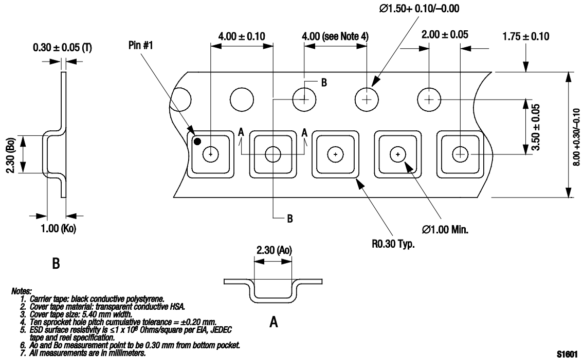
Figure 11. CLA4608-085LF Tape and Reel Dimensions
