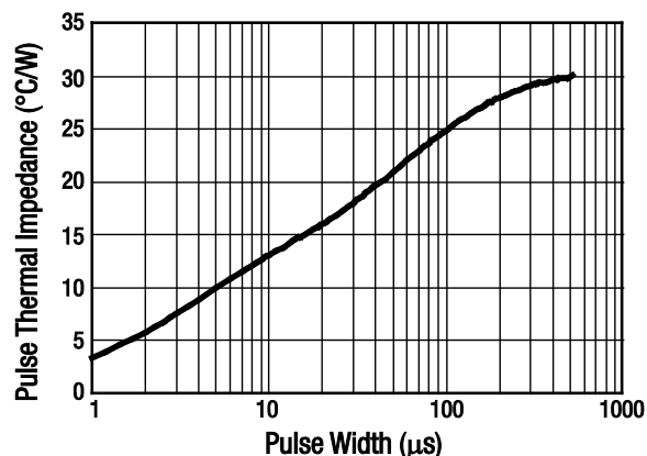
Figure 5. Typical Pulse Thermal Impedance
