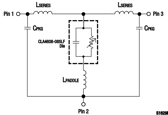
Figure 7. CLA4608-085LF Electrically Equivalent Circuit
