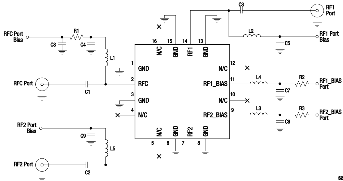
Figure 16. Evaluation Board Schematic
